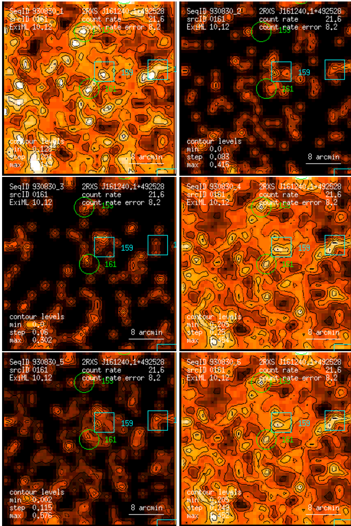
Figure 161: RASS 930830: detection 0161: band rate images, Gaussian filter: (1) PSPC channels 11 – 41, (2) 52 – 90, (3) 91 – 201, (4) 11 – 235, (5) 52 – 201, (6) 11 – 201. Broad band rates in counts/ks. Band rate contour levels in counts/ks/arcmin 2 .
