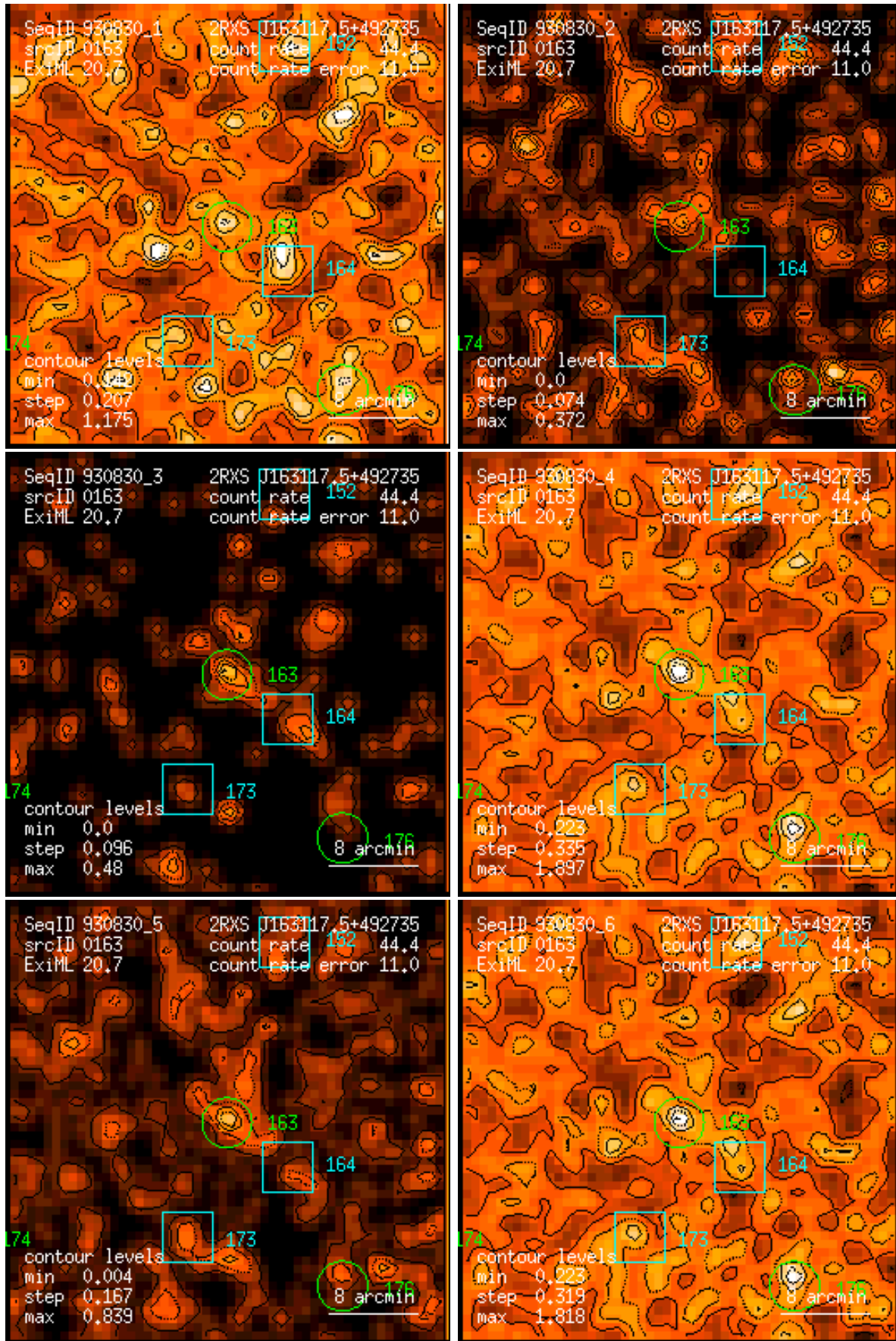
Figure 163: RASS 930830: detection 0163: band rate images, Gaussian filter: (1) PSPC channels 11 – 41, (2) 52 – 90, (3) 91 – 201, (4) 11 – 235, (5) 52 – 201, (6) 11 – 201. Broad band rates in counts/ks. Band rate contour levels in counts/ks/arcmin 2 .
