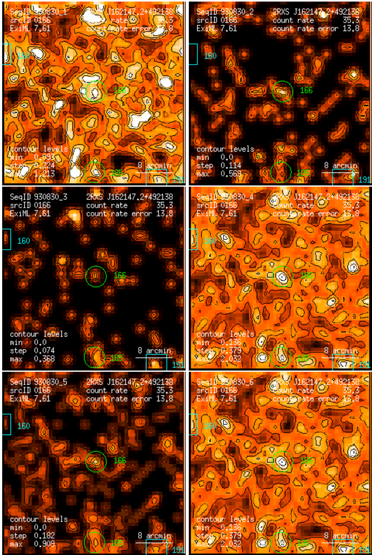
Figure 166: RASS 930830: detection 0166: band rate images, Gaussian filter: (1) PSPC channels 11 – 41, (2) 52 – 90, (3) 91 – 201, (4) 11 – 235, (5) 52 – 201, (6) 11 – 201. Broad band rates in counts/ks. Band rate contour levels in counts/ks/arcmin 2 .
