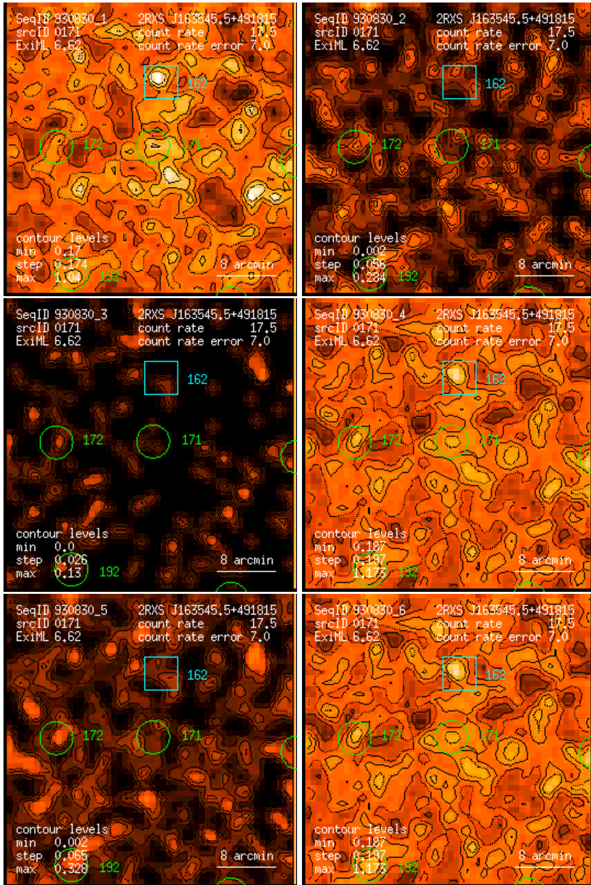
Figure 171: RASS 930830: detection 0171: band rate images, Gaussian filter: (1) PSPC channels 11 – 41, (2) 52 – 90, (3) 91 – 201, (4) 11 – 235, (5) 52 – 201, (6) 11 – 201. Broad band rates in counts/ks. Band rate contour levels in counts/ks/arcmin 2 .
