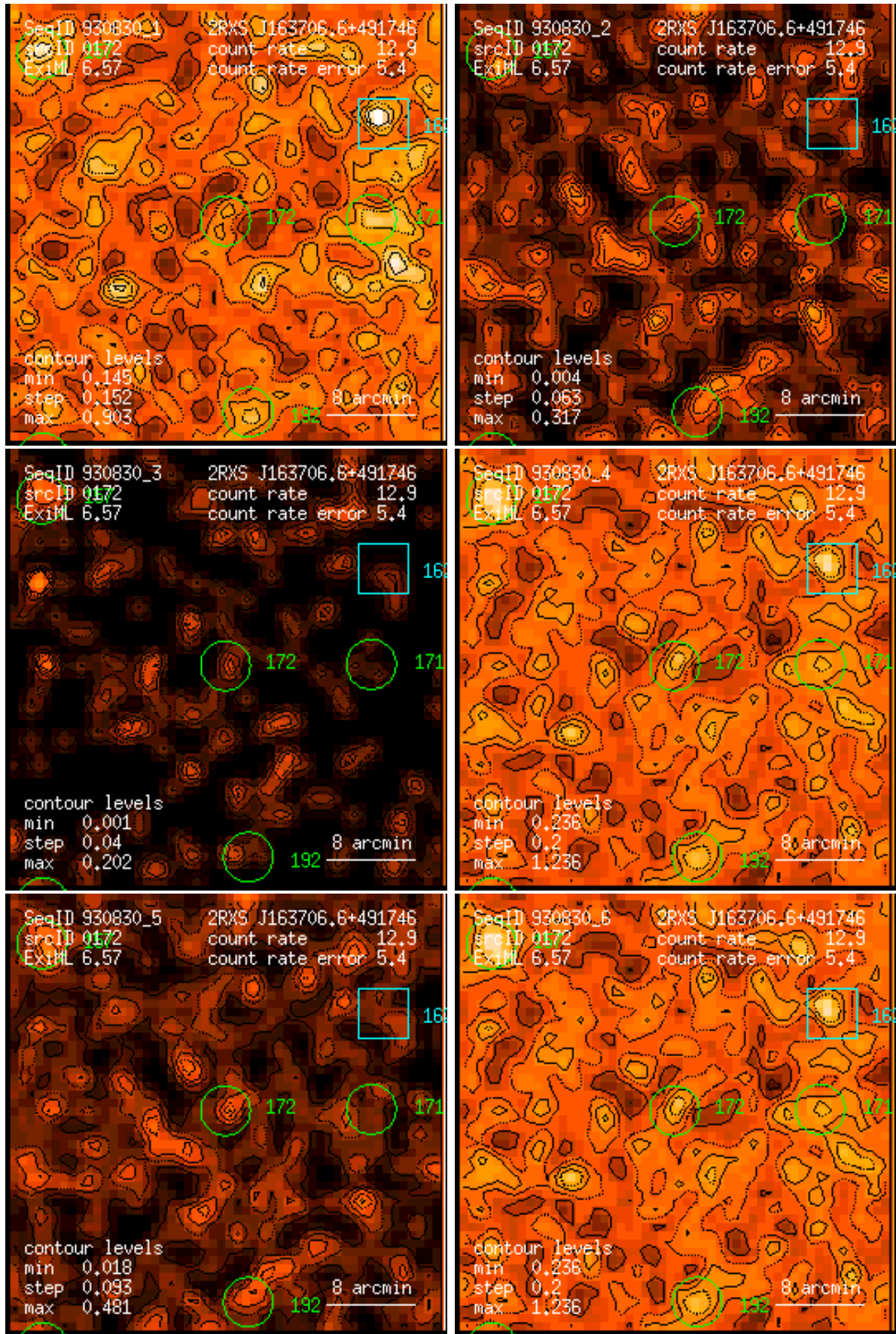
Figure 172: RASS 930830: detection 0172: band rate images, Gaussian filter: (1) PSPC channels 11 – 41, (2) 52 – 90, (3) 91 – 201, (4) 11 – 235, (5) 52 – 201, (6) 11 – 201. Broad band rates in counts/ks. Band rate contour levels in counts/ks/arcmin 2 .
