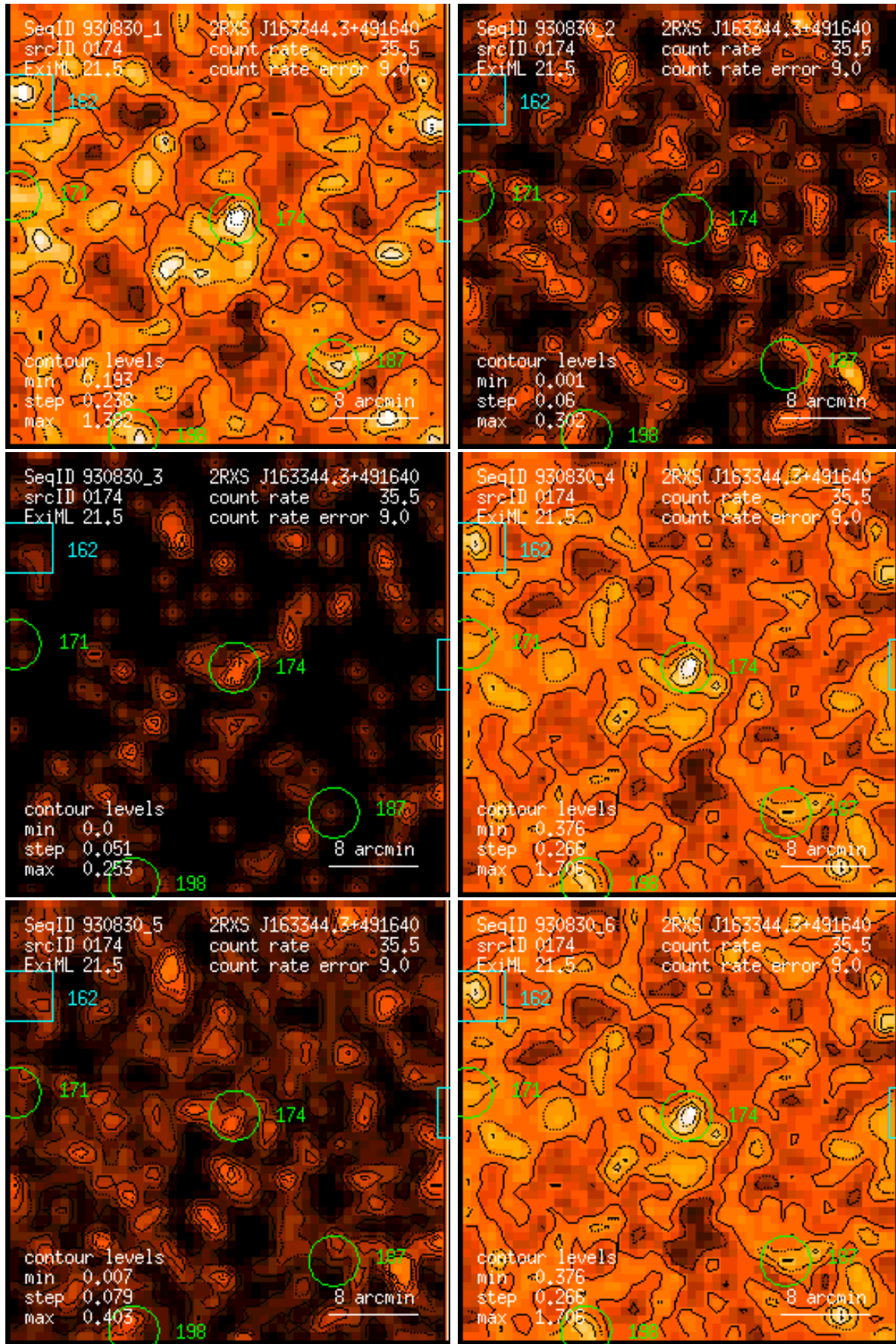
Figure 174: RASS 930830: detection 0174: band rate images, Gaussian filter: (1) PSPC channels 11 – 41, (2) 52 – 90, (3) 91 – 201, (4) 11 – 235, (5) 52 – 201, (6) 11 – 201. Broad band rates in counts/ks. Band rate contour levels in counts/ks/arcmin 2 .
