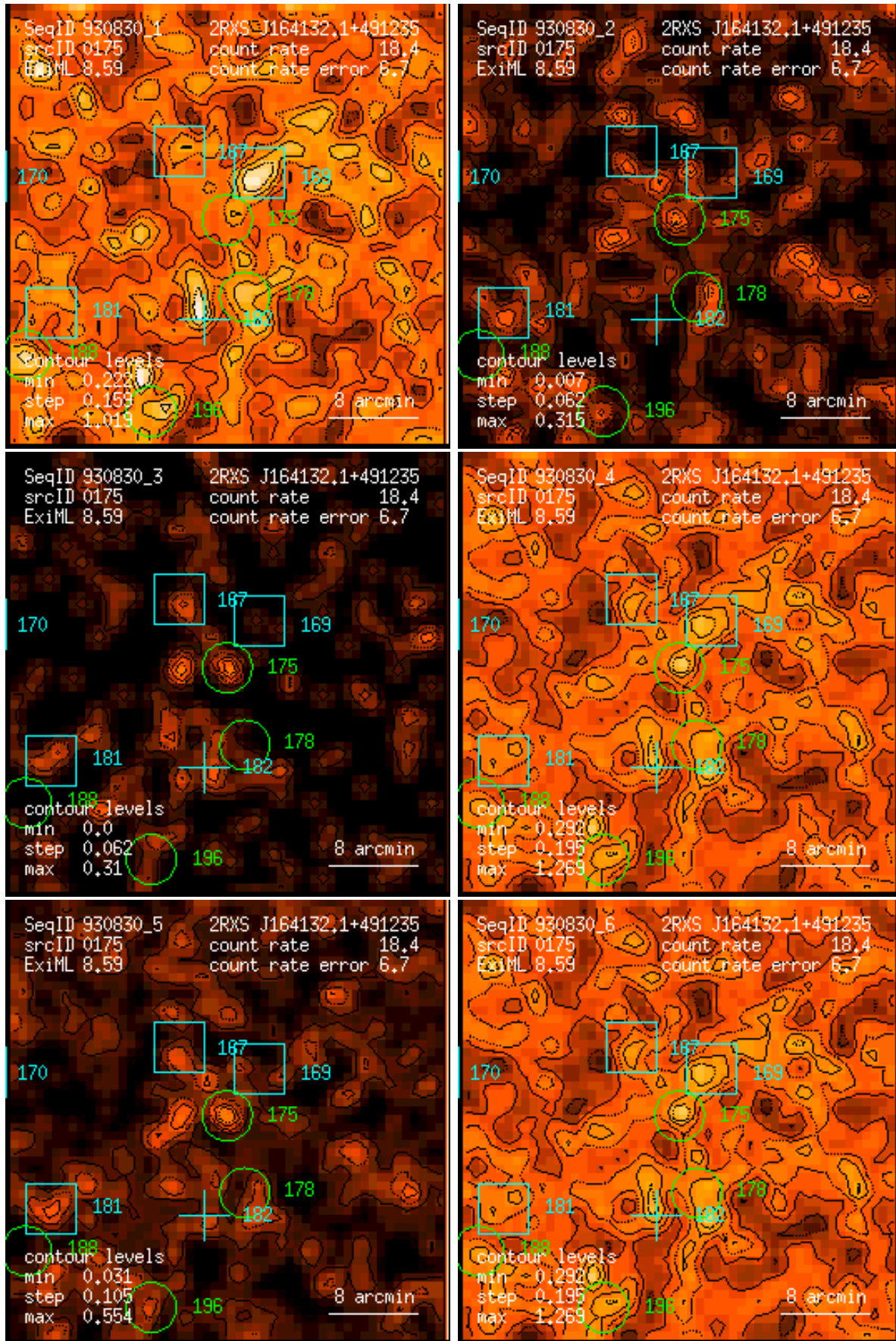
Figure 175: RASS 930830: detection 0175: band rate images, Gaussian filter: (1) PSPC channels 11 – 41, (2) 52 – 90, (3) 91 – 201, (4) 11 – 235, (5) 52 – 201, (6) 11 – 201. Broad band rates in counts/ks. Band rate contour levels in counts/ks/arcmin 2 .
