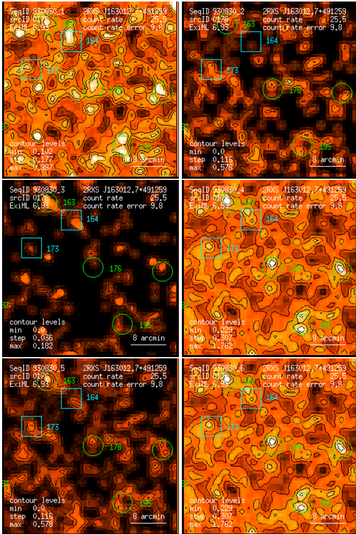
Figure 176: RASS 930830: detection 0176: band rate images, Gaussian filter: (1) PSPC channels 11 – 41, (2) 52 – 90, (3) 91 – 201, (4) 11 – 235, (5) 52 – 201, (6) 11 – 201. Broad band rates in counts/ks. Band rate contour levels in counts/ks/arcmin 2 .
