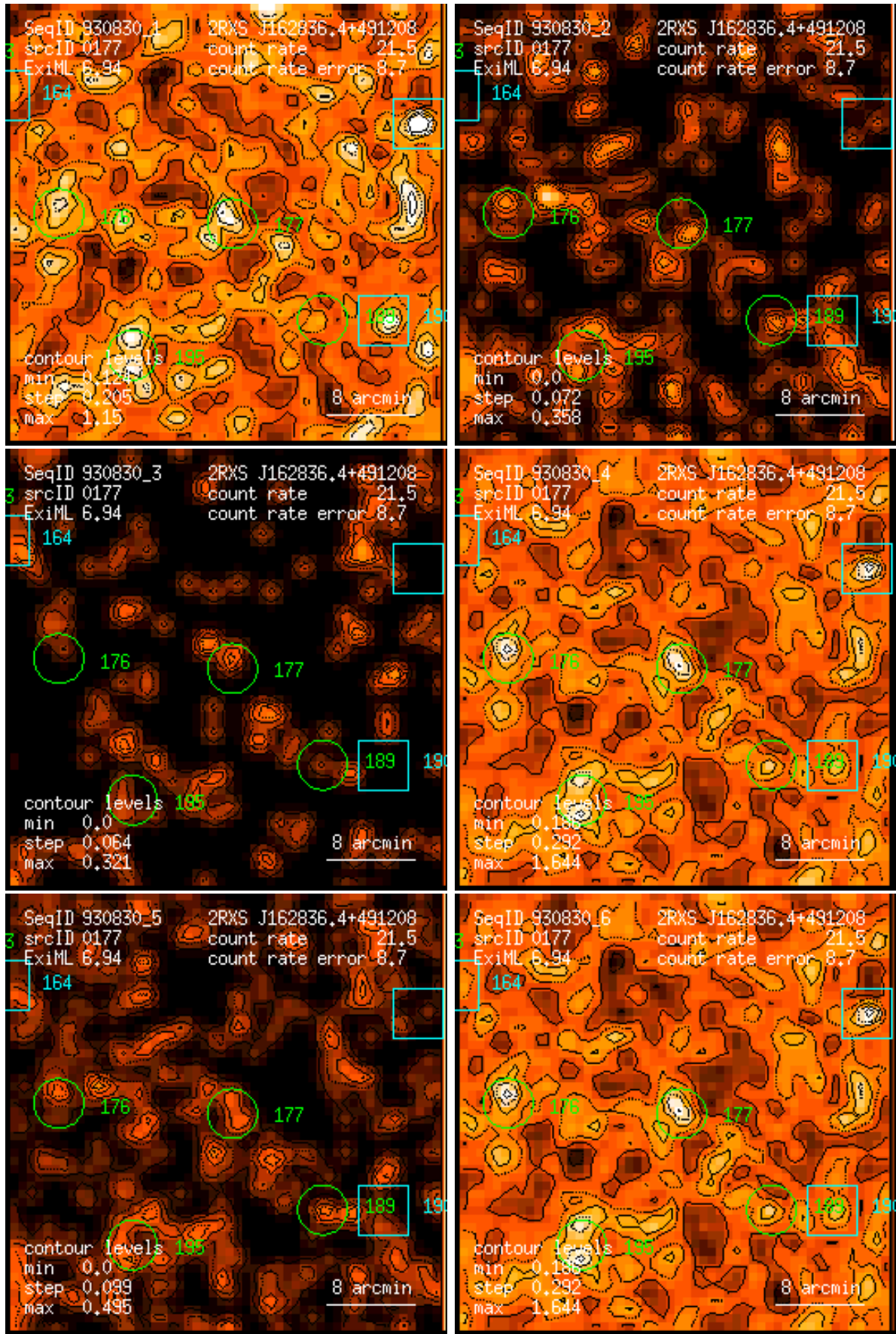
Figure 177: RASS 930830: detection 0177: band rate images, Gaussian filter: (1) PSPC channels 11 – 41, (2) 52 – 90, (3) 91 – 201, (4) 11 – 235, (5) 52 – 201, (6) 11 – 201. Broad band rates in counts/ks. Band rate contour levels in counts/ks/arcmin 2 .
