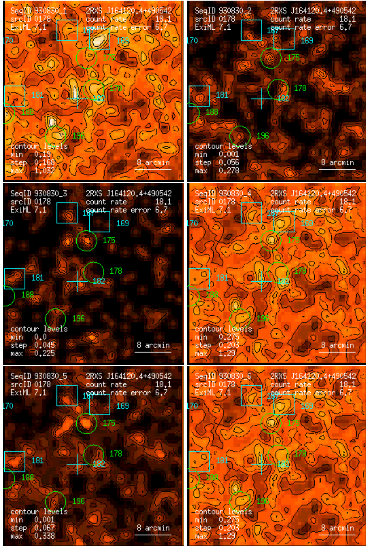
Figure 178: RASS 930830: detection 0178: band rate images, Gaussian filter: (1) PSPC channels 11 – 41, (2) 52 – 90, (3) 91 – 201, (4) 11 – 235, (5) 52 – 201, (6) 11 – 201. Broad band rates in counts/ks. Band rate contour levels in counts/ks/arcmin 2 .
