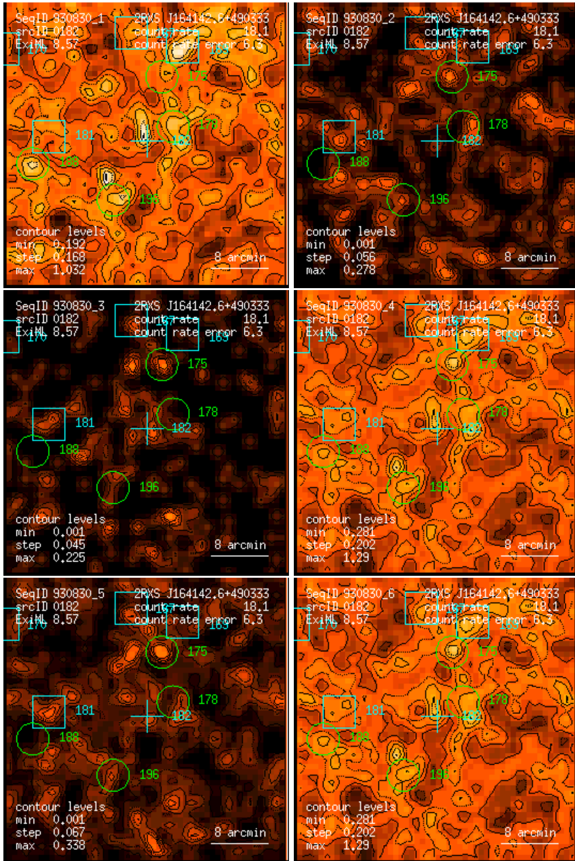
Figure 182: RASS 930830: detection 0182: band rate images, Gaussian filter: (1) PSPC channels 11 – 41, (2) 52 – 90, (3) 91 – 201, (4) 11 – 235, (5) 52 – 201, (6) 11 – 201. Broad band rates in counts/ks. Band rate contour levels in counts/ks/arcmin 2 .
