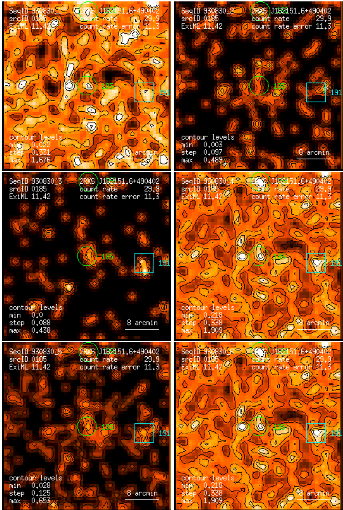
Figure 185: RASS 930830: detection 0185: band rate images, Gaussian filter: (1) PSPC channels 11 – 41, (2) 52 – 90, (3) 91 – 201, (4) 11 – 235, (5) 52 – 201, (6) 11 – 201. Broad band rates in counts/ks. Band rate contour levels in counts/ks/arcmin 2 .
