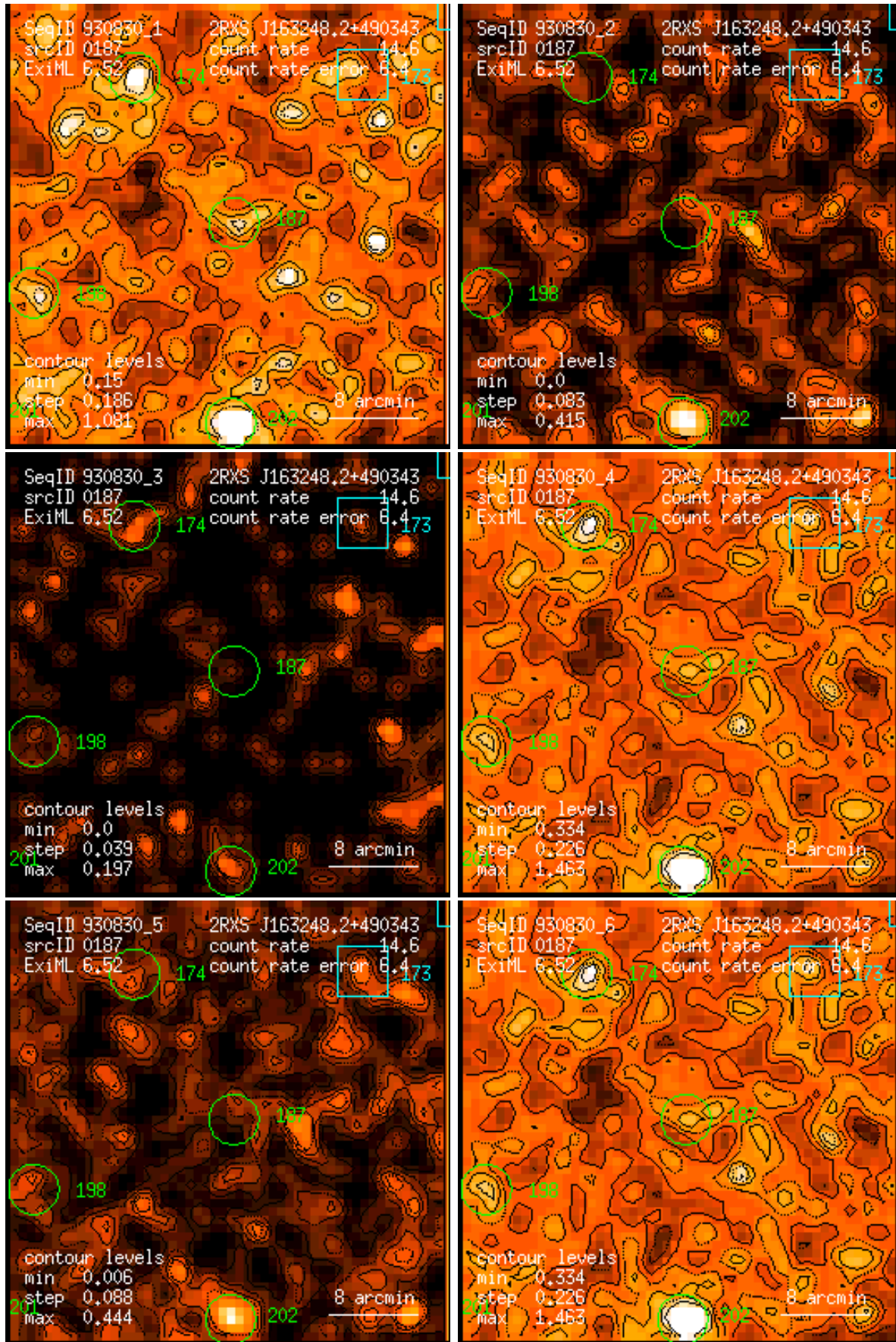
Figure 187: RASS 930830: detection 0187: band rate images, Gaussian filter: (1) PSPC channels 11 – 41, (2) 52 – 90, (3) 91 – 201, (4) 11 – 235, (5) 52 – 201, (6) 11 – 201. Broad band rates in counts/ks. Band rate contour levels in counts/ks/arcmin 2 .
