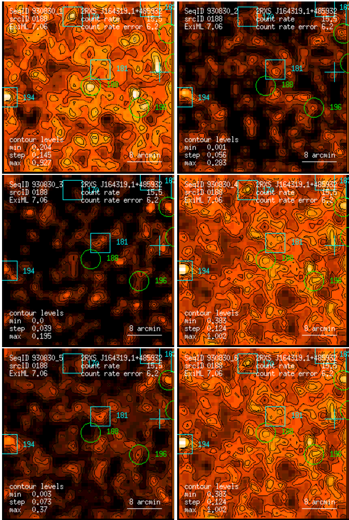
Figure 188: RASS 930830: detection 0188: band rate images, Gaussian filter: (1) PSPC channels 11 – 41, (2) 52 – 90, (3) 91 – 201, (4) 11 – 235, (5) 52 – 201, (6) 11 – 201. Broad band rates in counts/ks. Band rate contour levels in counts/ks/arcmin 2 .
