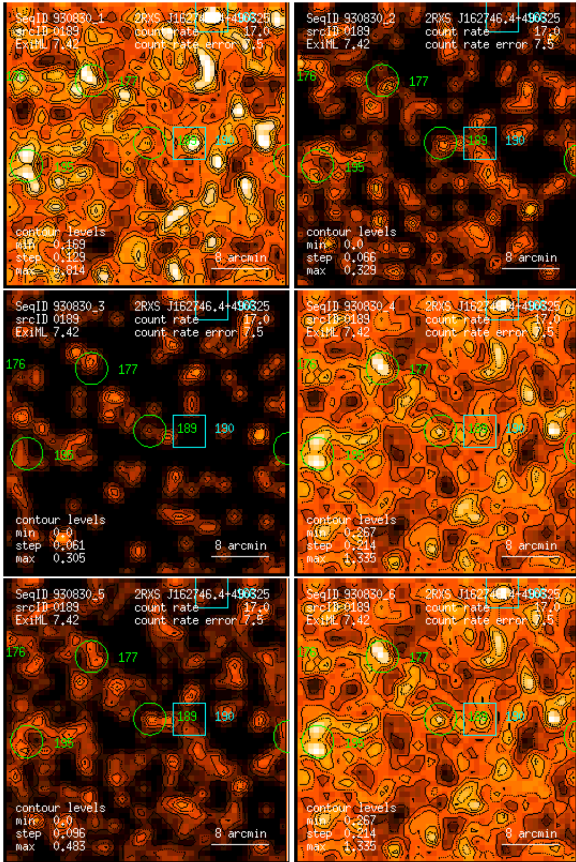
Figure 189: RASS 930830: detection 0189: band rate images, Gaussian filter: (1) PSPC channels 11 – 41, (2) 52 – 90, (3) 91 – 201, (4) 11 – 235, (5) 52 – 201, (6) 11 – 201. Broad band rates in counts/ks. Band rate contour levels in counts/ks/arcmin 2 .
