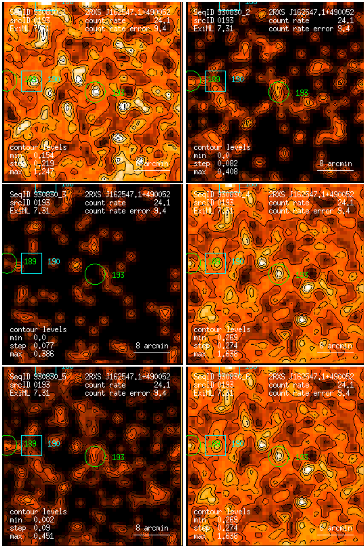
Figure 193: RASS 930830: detection 0193: band rate images, Gaussian filter: (1) PSPC channels 11 – 41, (2) 52 – 90, (3) 91 – 201, (4) 11 – 235, (5) 52 – 201, (6) 11 – 201. Broad band rates in counts/ks. Band rate contour levels in counts/ks/arcmin 2 .
