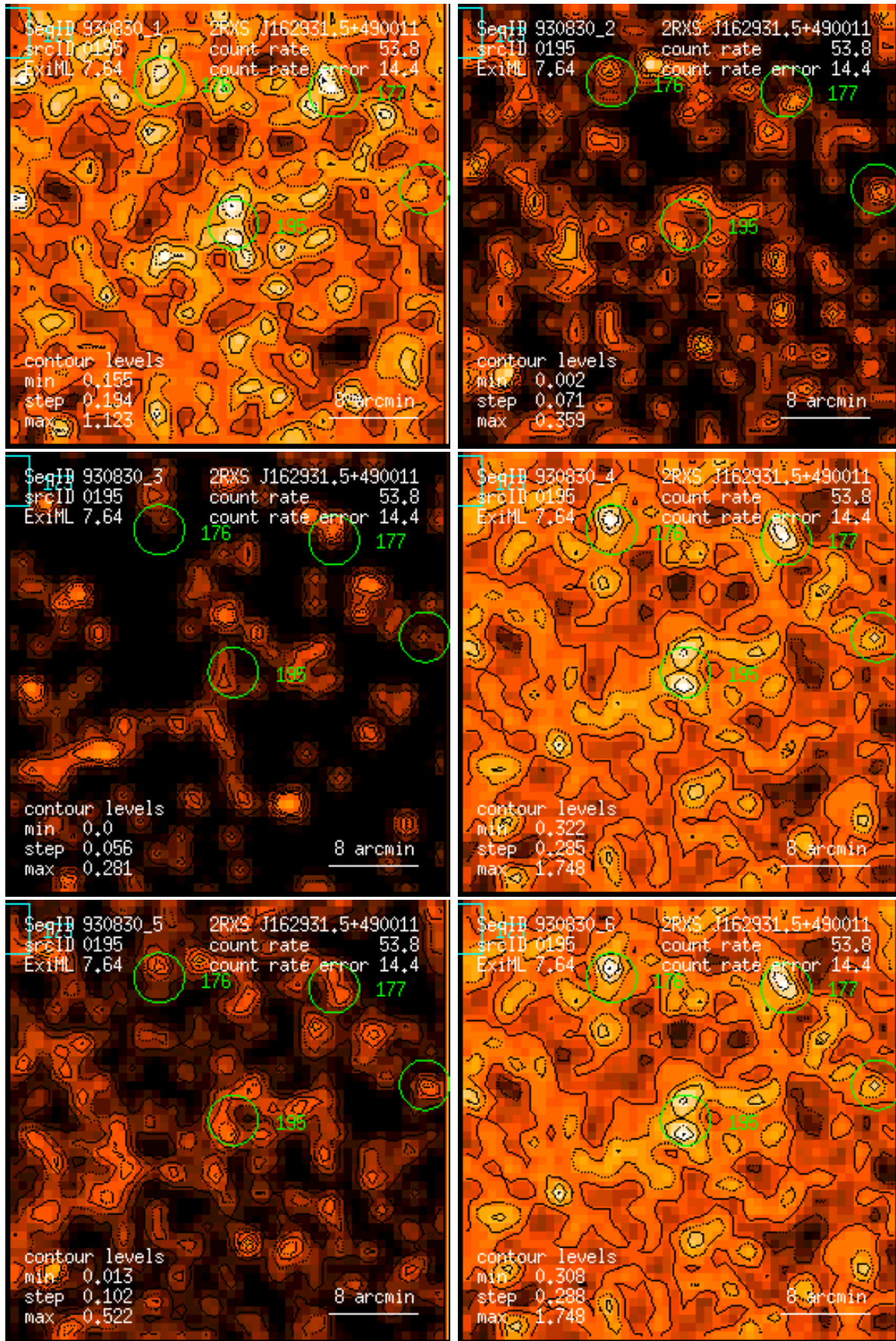
Figure 195: RASS 930830: detection 0195: band rate images, Gaussian filter: (1) PSPC channels 11 – 41, (2) 52 – 90, (3) 91 – 201, (4) 11 – 235, (5) 52 – 201, (6) 11 – 201. Broad band rates in counts/ks. Band rate contour levels in counts/ks/arcmin 2 .
