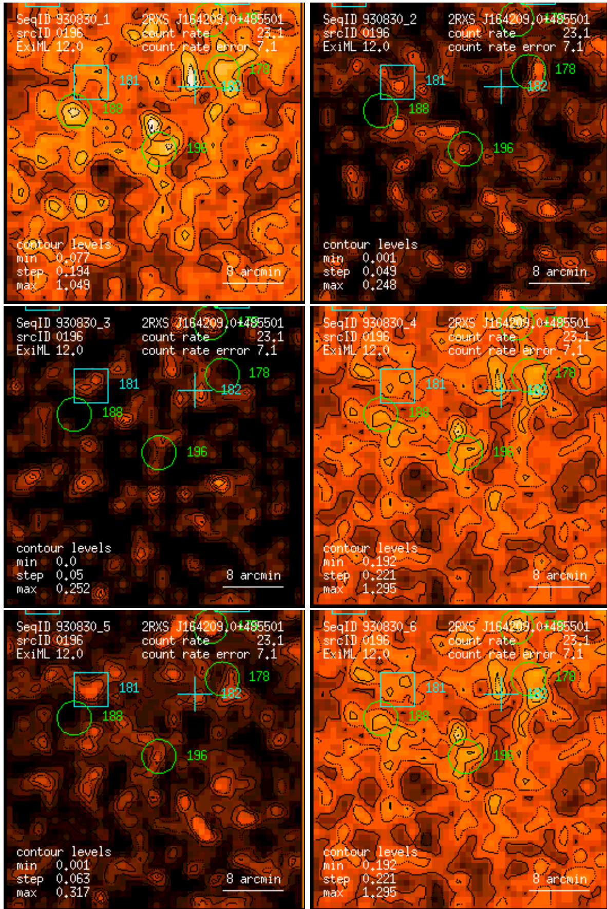
Figure 196: RASS 930830: detection 0196: band rate images, Gaussian filter: (1) PSPC channels 11 – 41, (2) 52 – 90, (3) 91 – 201, (4) 11 – 235, (5) 52 – 201, (6) 11 – 201. Broad band rates in counts/ks. Band rate contour levels in counts/ks/arcmin 2 .
