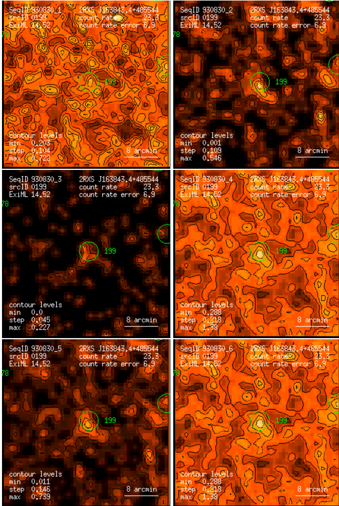
Figure 199: RASS 930830: detection 0199: band rate images, Gaussian filter: (1) PSPC channels 11 – 41, (2) 52 – 90, (3) 91 – 201, (4) 11 – 235, (5) 52 – 201, (6) 11 – 201. Broad band rates in counts/ks. Band rate contour levels in counts/ks/arcmin 2 .
