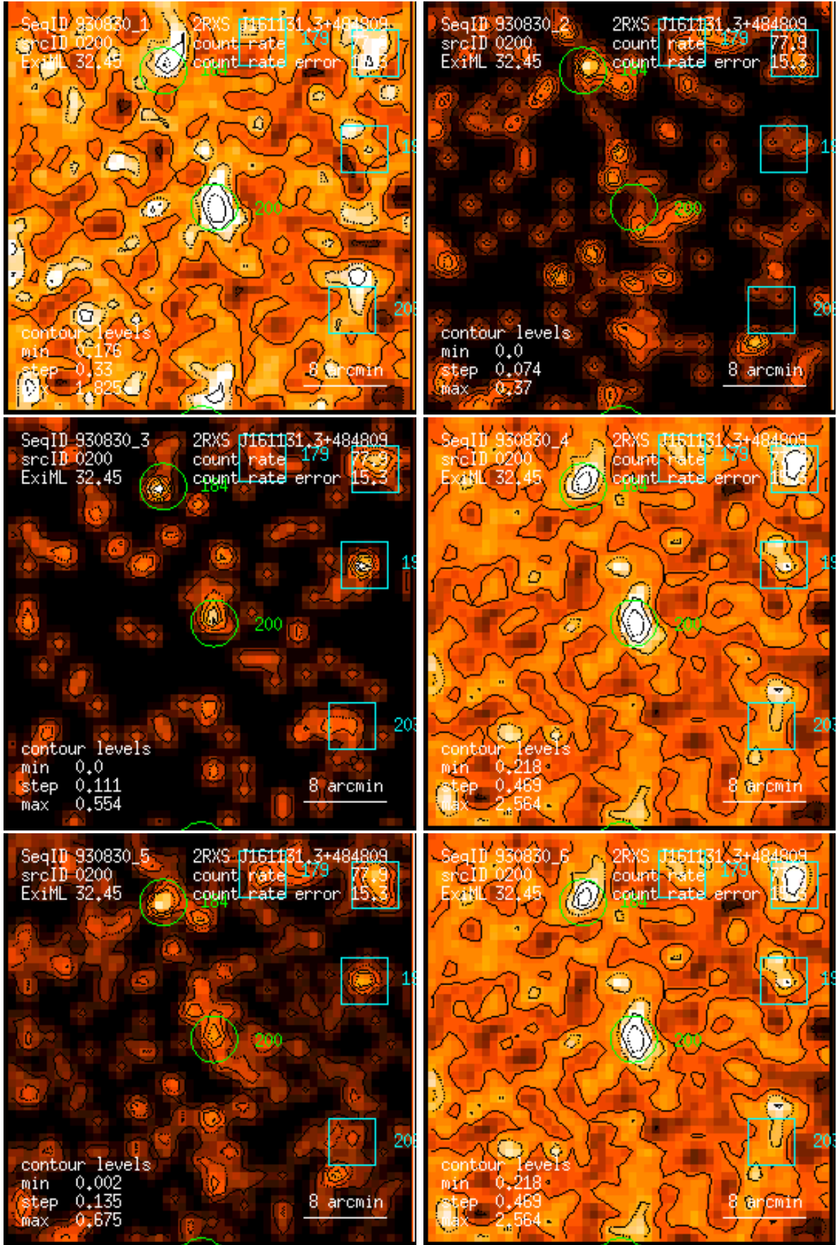
Figure 200: RASS 930830: detection 0200: band rate images, Gaussian filter: (1) PSPC channels 11 – 41, (2) 52 – 90, (3) 91 – 201, (4) 11 – 235, (5) 52 – 201, (6) 11 – 201. Broad band rates in counts/ks. Band rate contour levels in counts/ks/arcmin 2 .
