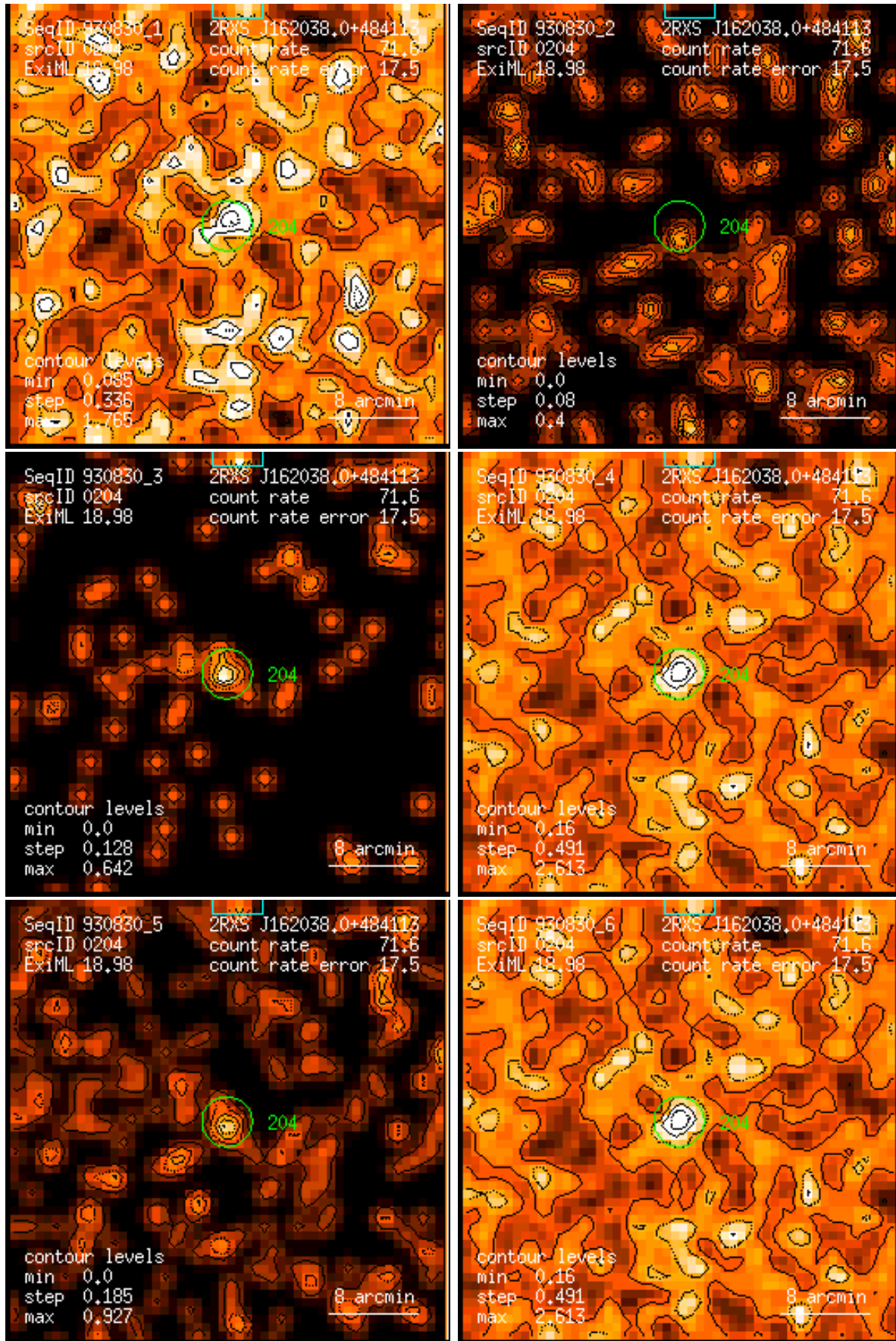
Figure 204: RASS 930830: detection 0204: band rate images, Gaussian filter: (1) PSPC channels 11 – 41, (2) 52 – 90, (3) 91 – 201, (4) 11 – 235, (5) 52 – 201, (6) 11 – 201. Broad band rates in counts/ks. Band rate contour levels in counts/ks/arcmin 2 .
