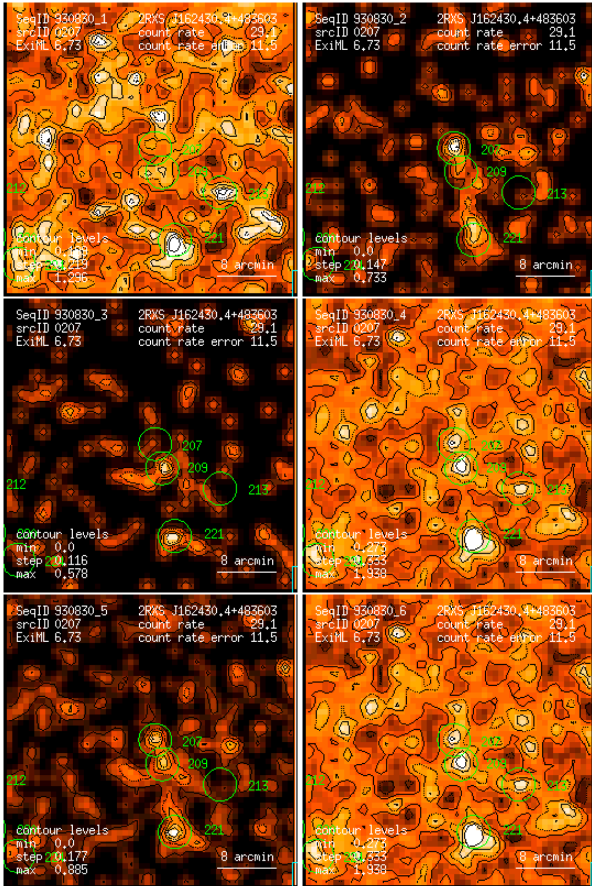
Figure 207: RASS 930830: detection 0207: band rate images, Gaussian filter: (1) PSPC channels 11 – 41, (2) 52 – 90, (3) 91 – 201, (4) 11 – 235, (5) 52 – 201, (6) 11 – 201. Broad band rates in counts/ks. Band rate contour levels in counts/ks/arcmin 2 .
