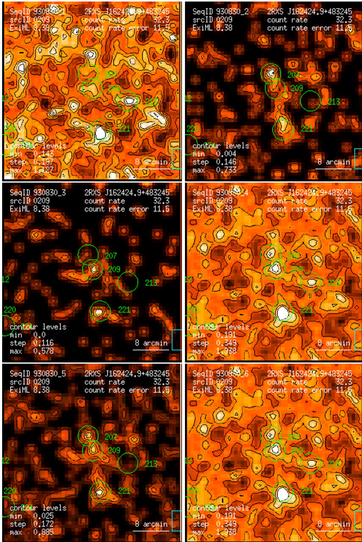
Figure 209: RASS 930830: detection 0209: band rate images, Gaussian filter: (1) PSPC channels 11 – 41, (2) 52 – 90, (3) 91 – 201, (4) 11 – 235, (5) 52 – 201, (6) 11 – 201. Broad band rates in counts/ks. Band rate contour levels in counts/ks/arcmin 2 .
