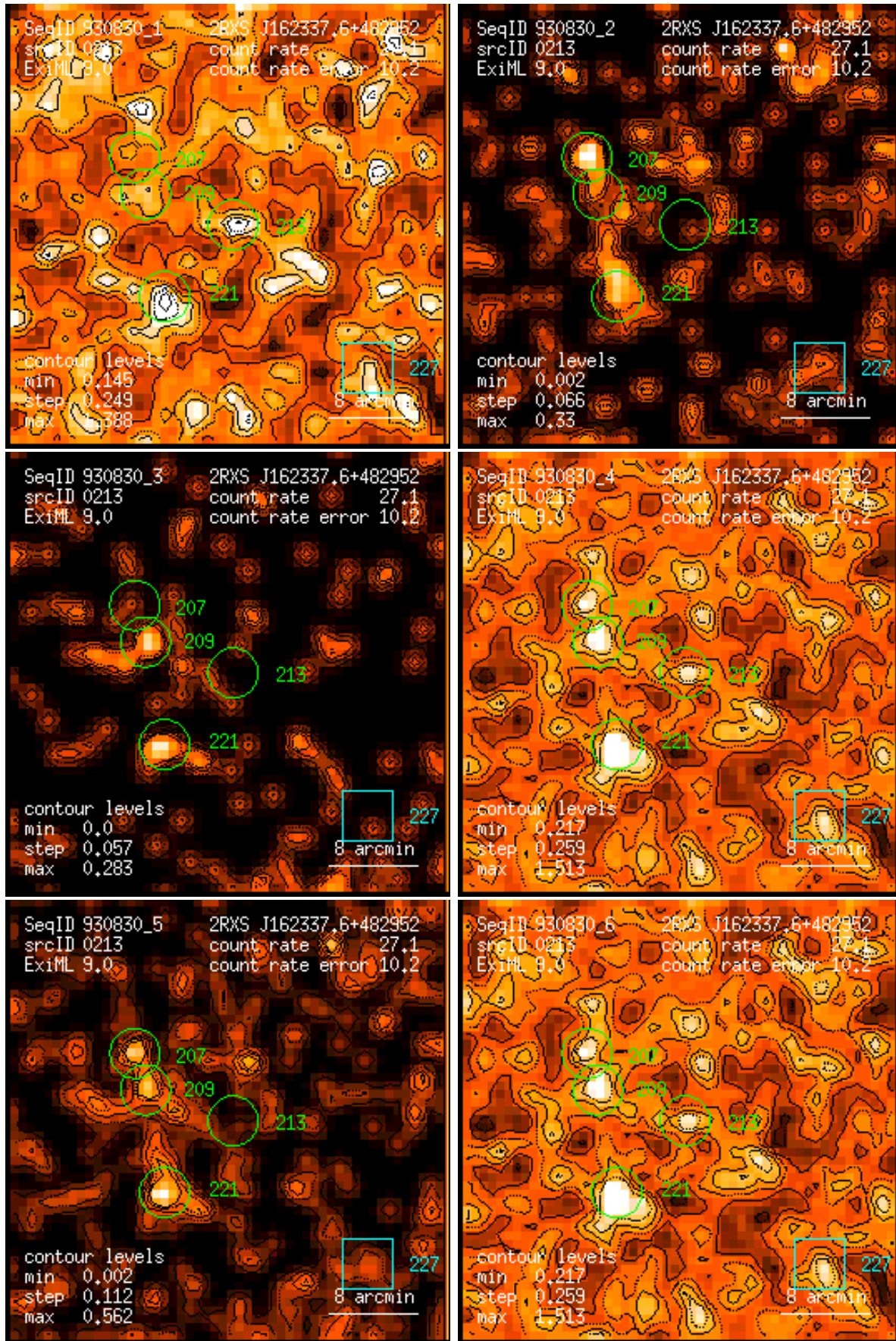
Figure 213: RASS 930830: detection 0213: band rate images, Gaussian filter: (1) PSPC channels 11 – 41, (2) 52 – 90, (3) 91 – 201, (4) 11 – 235, (5) 52 – 201, (6) 11 – 201. Broad band rates in counts/ks. Band rate contour levels in counts/ks/arcmin 2 .
