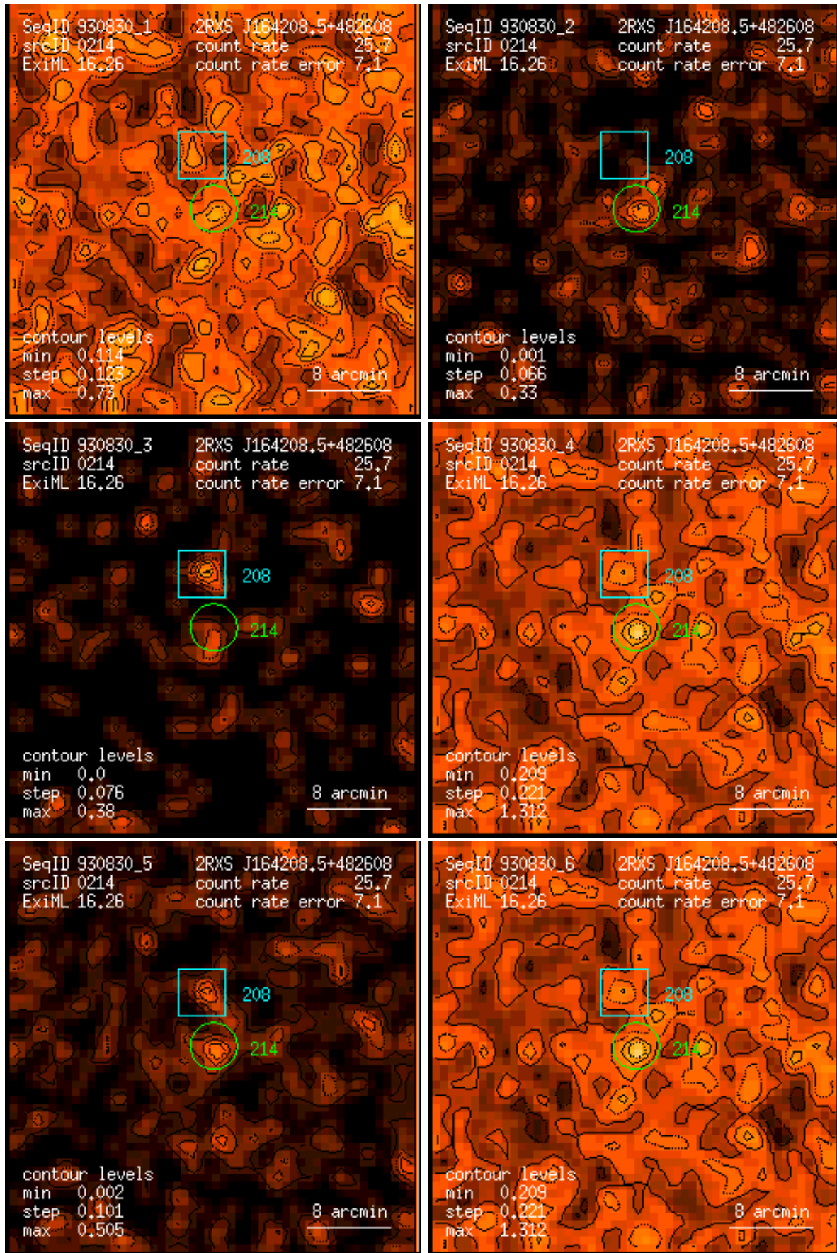
Figure 214: RASS 930830: detection 0214: band rate images, Gaussian filter: (1) PSPC channels 11 – 41, (2) 52 – 90, (3) 91 – 201, (4) 11 – 235, (5) 52 – 201, (6) 11 – 201. Broad band rates in counts/ks. Band rate contour levels in counts/ks/arcmin 2 .
