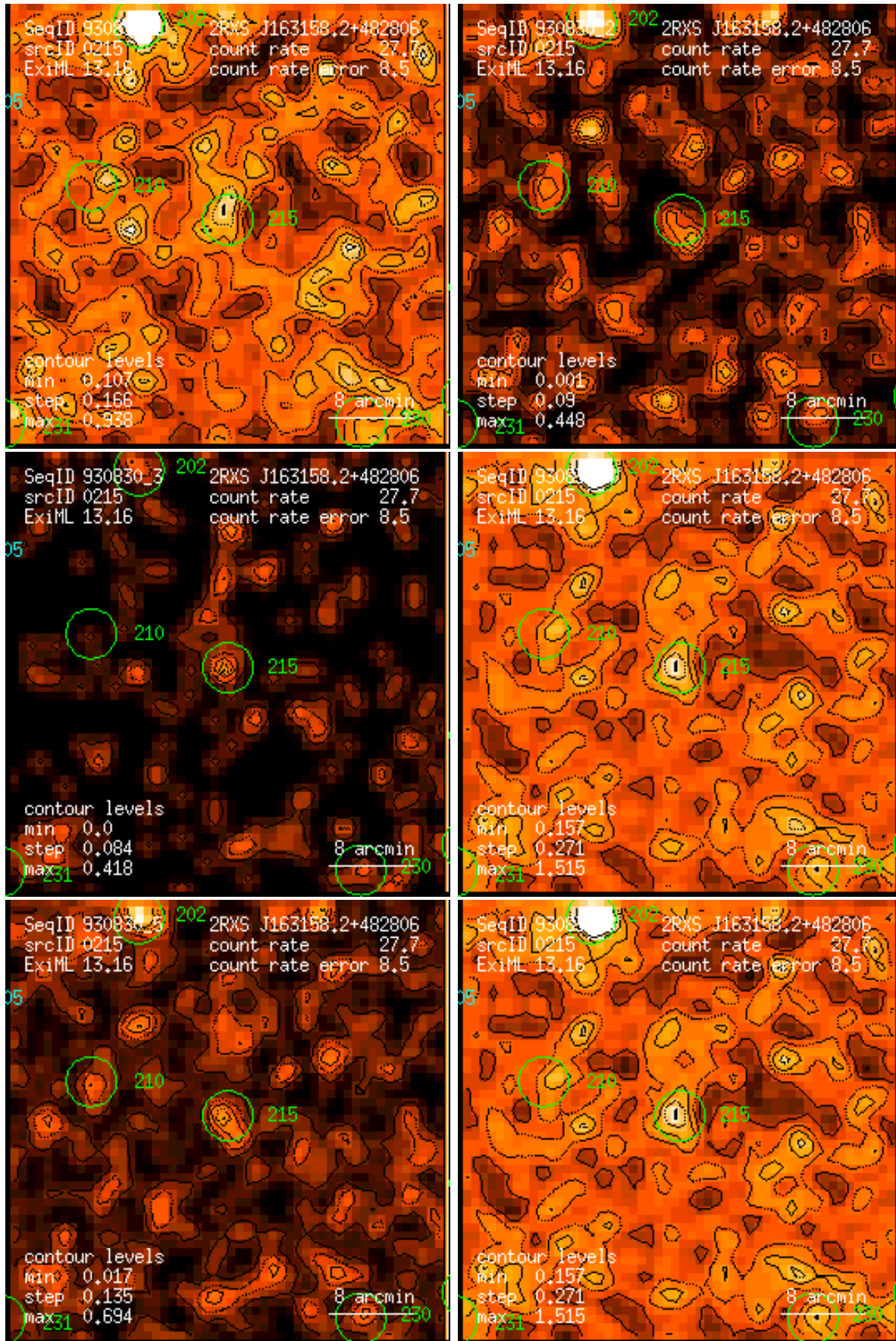
Figure 215: RASS 930830: detection 0215: band rate images, Gaussian filter: (1) PSPC channels 11 – 41, (2) 52 – 90, (3) 91 – 201, (4) 11 – 235, (5) 52 – 201, (6) 11 – 201. Broad band rates in counts/ks. Band rate contour levels in counts/ks/arcmin 2 .
