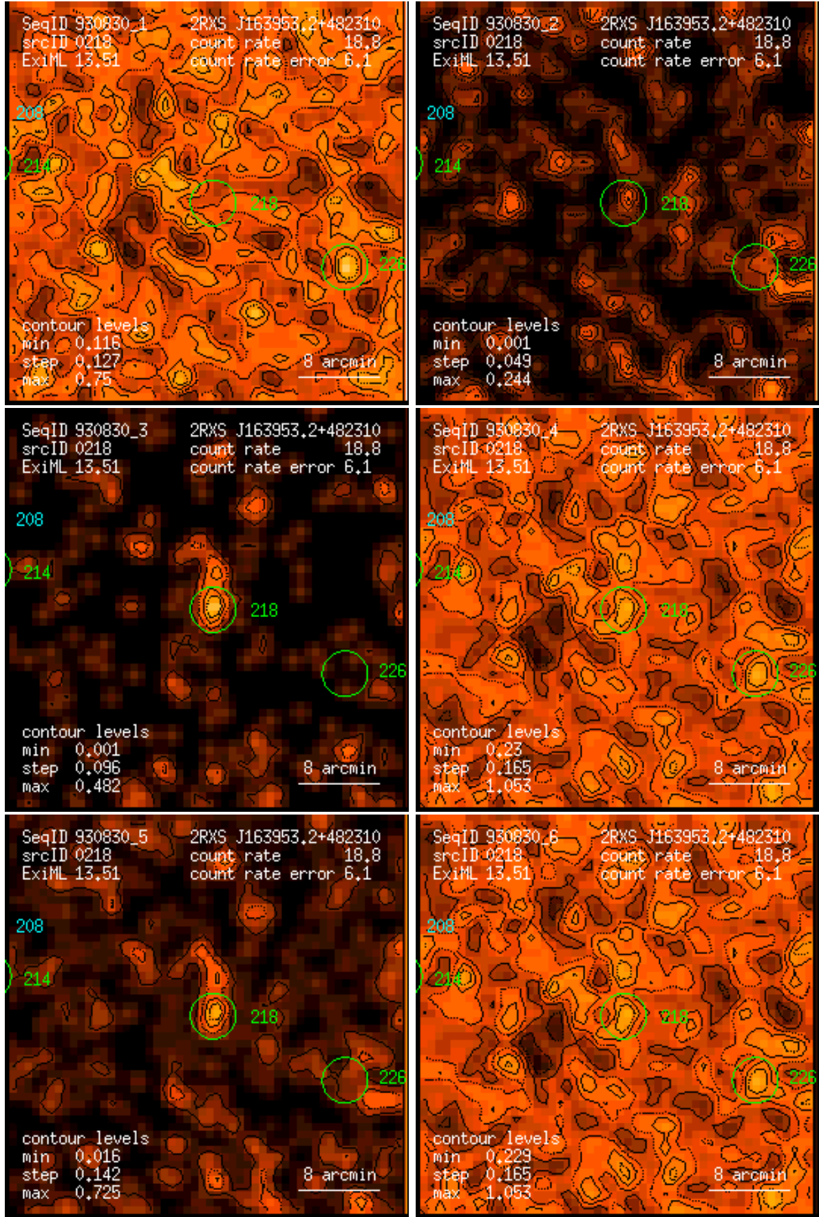
Figure 218: RASS 930830: detection 0218: band rate images, Gaussian filter: (1) PSPC channels 11 – 41, (2) 52 – 90, (3) 91 – 201, (4) 11 – 235, (5) 52 – 201, (6) 11 – 201. Broad band rates in counts/ks. Band rate contour levels in counts/ks/arcmin 2 .
