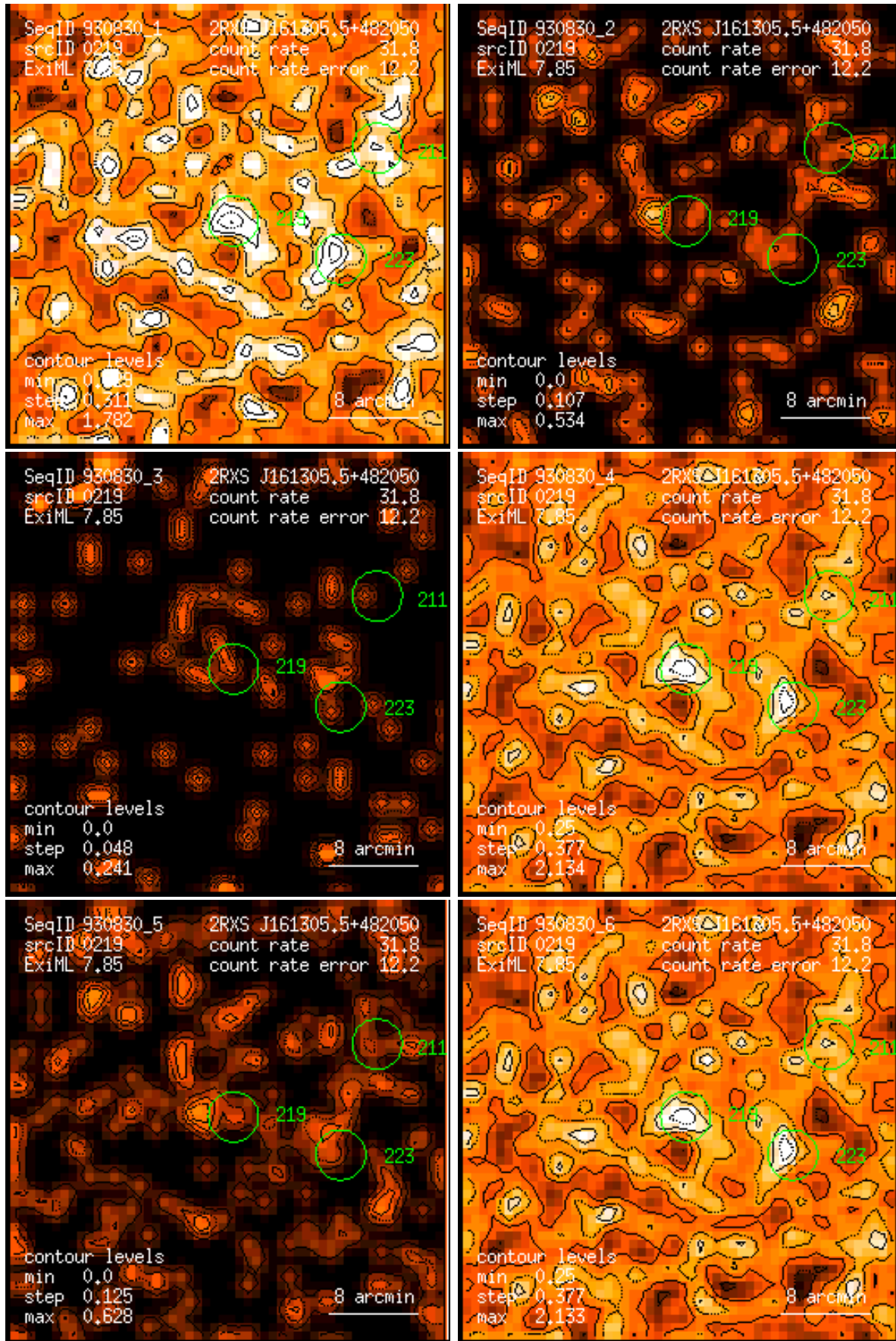
Figure 219: RASS 930830: detection 0219: band rate images, Gaussian filter: (1) PSPC channels 11 – 41, (2) 52 – 90, (3) 91 – 201, (4) 11 – 235, (5) 52 – 201, (6) 11 – 201. Broad band rates in counts/ks. Band rate contour levels in counts/ks/arcmin 2 .
