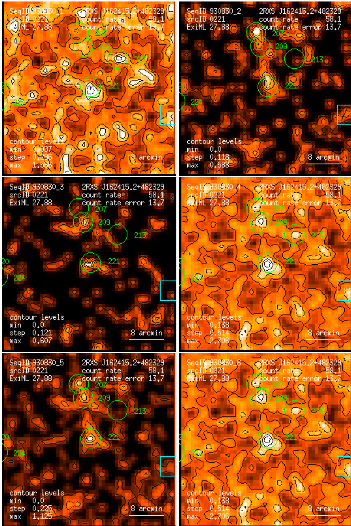
Figure 221: RASS 930830: detection 0221: band rate images, Gaussian filter: (1) PSPC channels 11 – 41, (2) 52 – 90, (3) 91 – 201, (4) 11 – 235, (5) 52 – 201, (6) 11 – 201. Broad band rates in counts/ks. Band rate contour levels in counts/ks/arcmin 2 .
