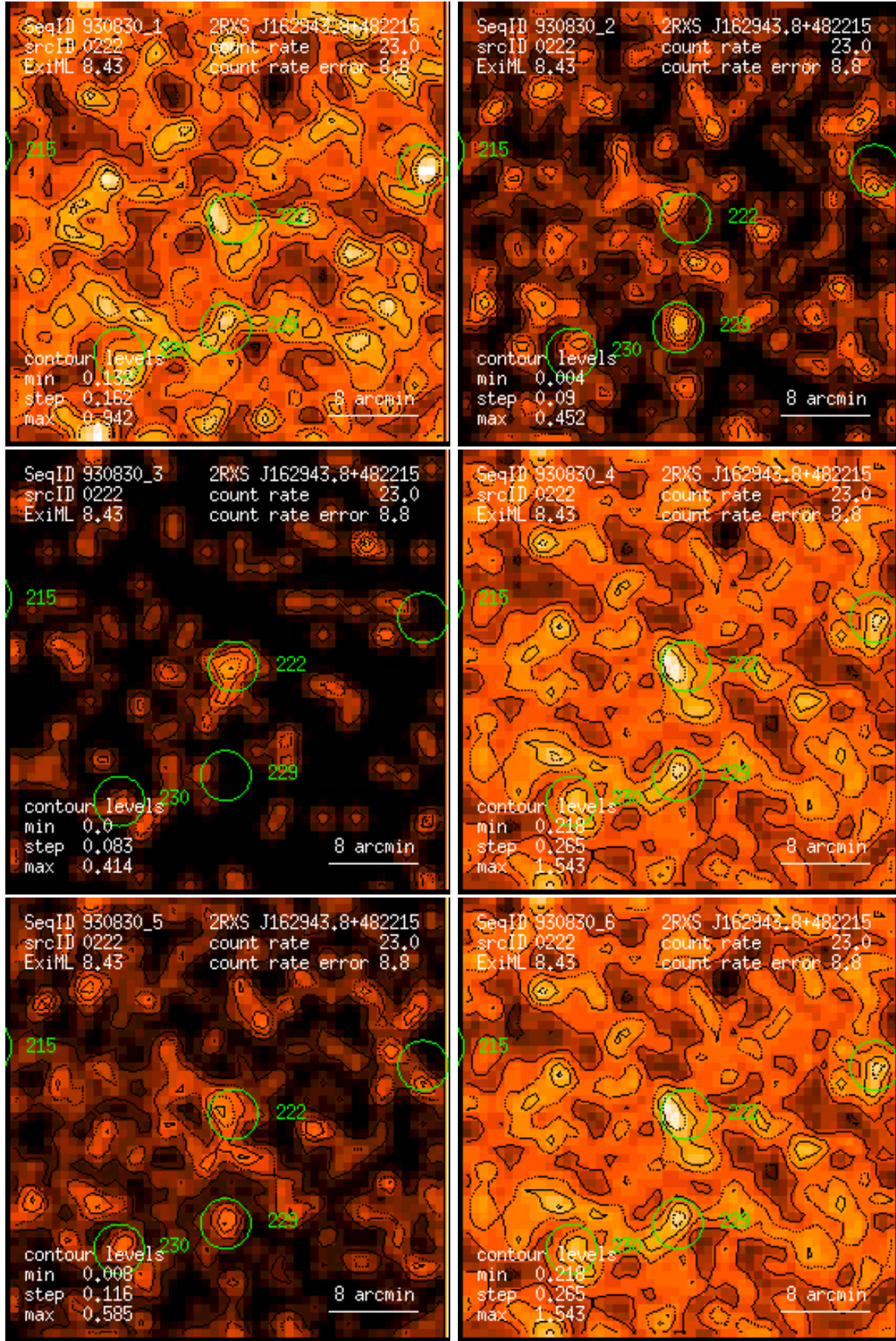
Figure 222: RASS 930830: detection 0222: band rate images, Gaussian filter: (1) PSPC channels 11 – 41, (2) 52 – 90, (3) 91 – 201, (4) 11 – 235, (5) 52 – 201, (6) 11 – 201. Broad band rates in counts/ks. Band rate contour levels in counts/ks/arcmin 2 .
