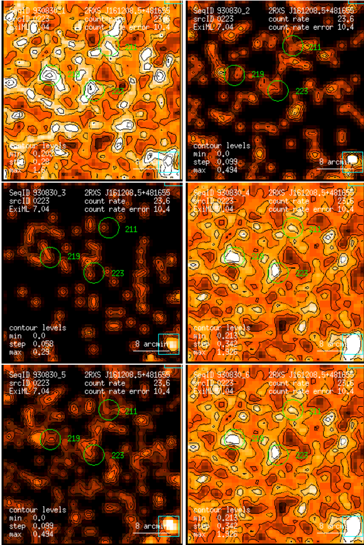
Figure 223: RASS 930830: detection 0223: band rate images, Gaussian filter: (1) PSPC channels 11 – 41, (2) 52 – 90, (3) 91 – 201, (4) 11 – 235, (5) 52 – 201, (6) 11 – 201. Broad band rates in counts/ks. Band rate contour levels in counts/ks/arcmin 2 .
