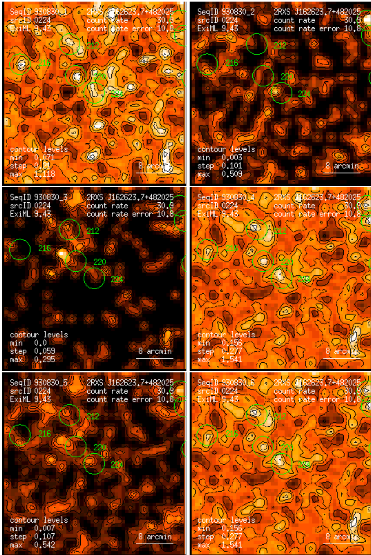
Figure 224: RASS 930830: detection 0224: band rate images, Gaussian filter: (1) PSPC channels 11 – 41, (2) 52 – 90, (3) 91 – 201, (4) 11 – 235, (5) 52 – 201, (6) 11 – 201. Broad band rates in counts/ks. Band rate contour levels in counts/ks/arcmin 2 .
