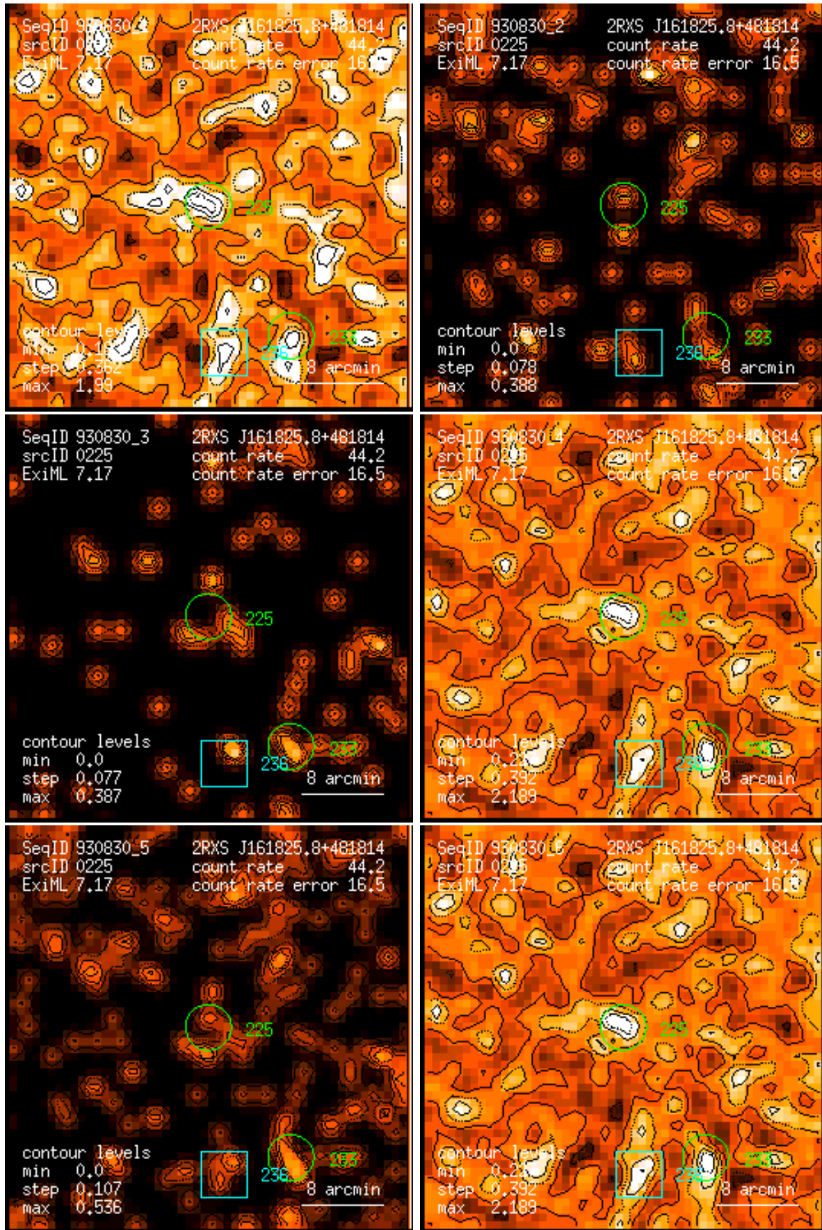
Figure 225: RASS 930830: detection 0225: band rate images, Gaussian filter: (1) PSPC channels 11 – 41, (2) 52 – 90, (3) 91 – 201, (4) 11 – 235, (5) 52 – 201, (6) 11 – 201. Broad band rates in counts/ks. Band rate contour levels in counts/ks/arcmin 2 .
