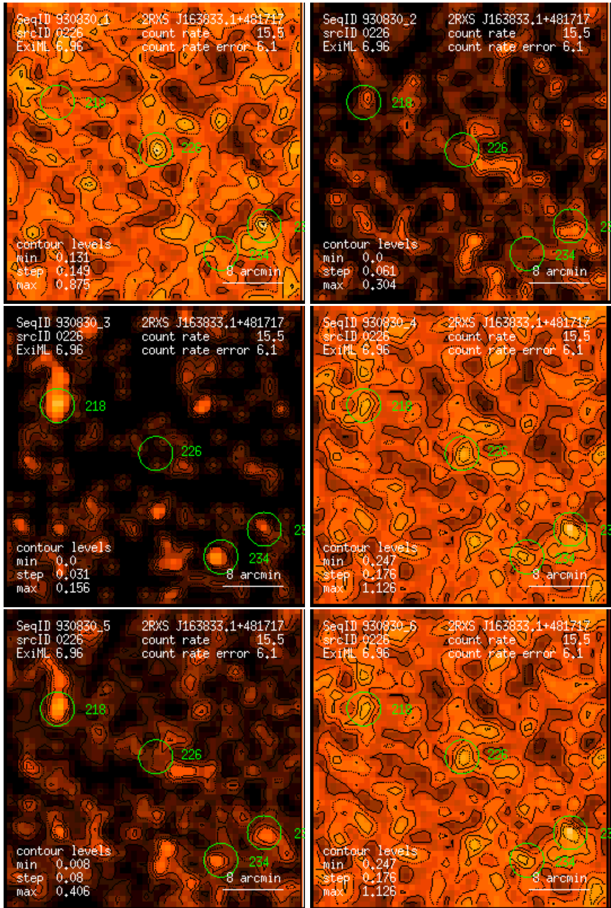
Figure 226: RASS 930830: detection 0226: band rate images, Gaussian filter: (1) PSPC channels 11 – 41, (2) 52 – 90, (3) 91 – 201, (4) 11 – 235, (5) 52 – 201, (6) 11 – 201. Broad band rates in counts/ks. Band rate contour levels in counts/ks/arcmin 2 .
