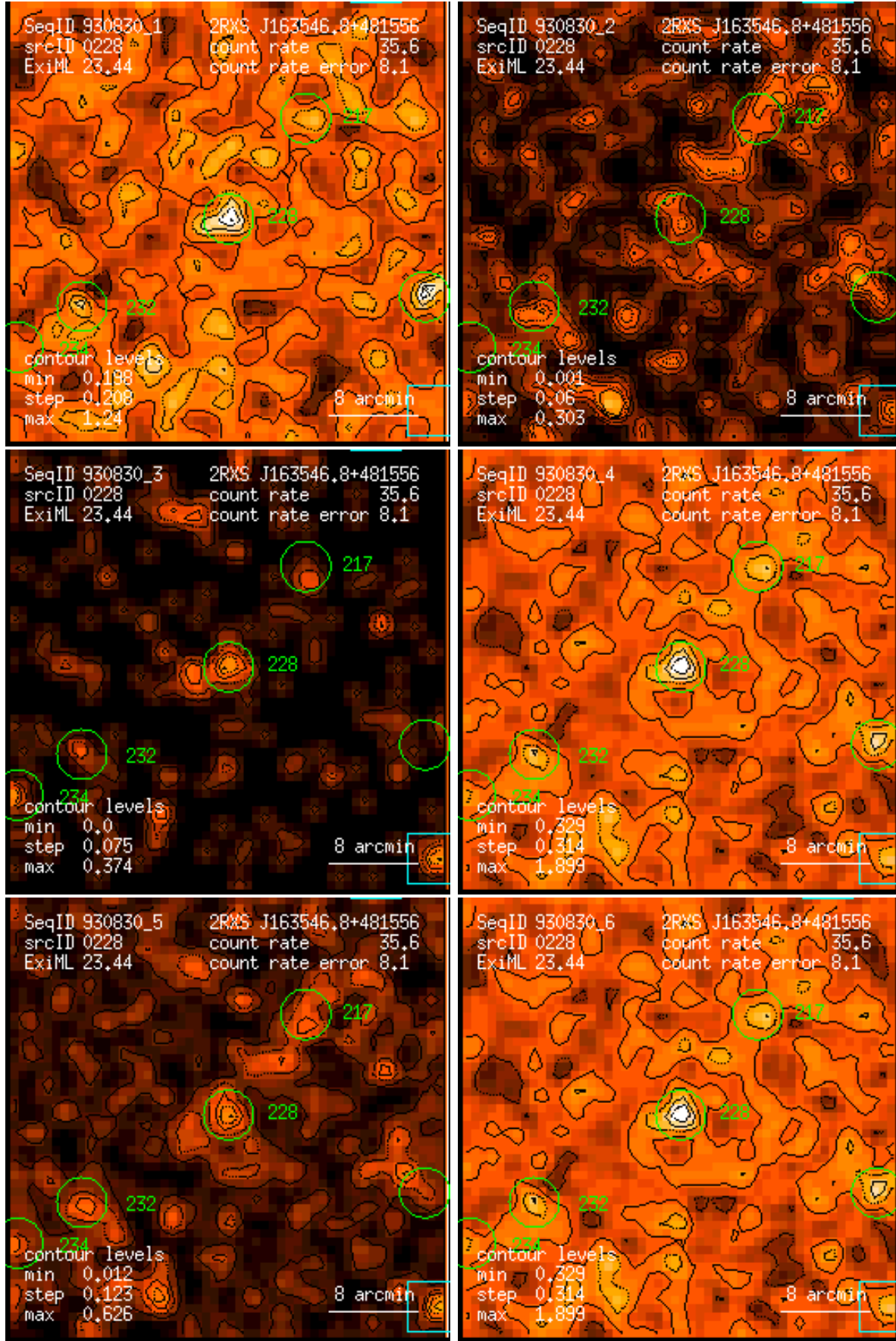
Figure 228: RASS 930830: detection 0228: band rate images, Gaussian filter: (1) PSPC channels 11 – 41, (2) 52 – 90, (3) 91 – 201, (4) 11 – 235, (5) 52 – 201, (6) 11 – 201. Broad band rates in counts/ks. Band rate contour levels in counts/ks/arcmin 2 .
