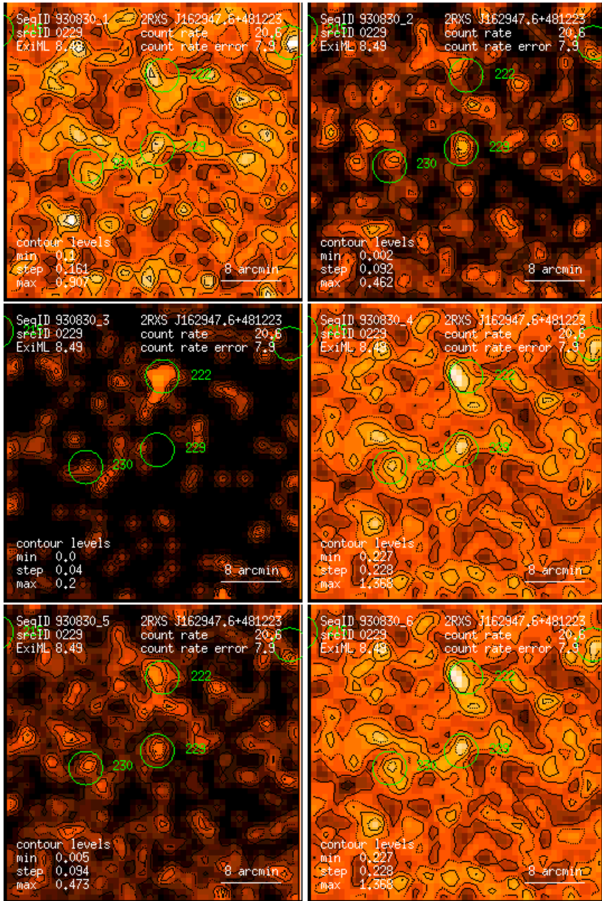
Figure 229: RASS 930830: detection 0229: band rate images, Gaussian filter: (1) PSPC channels 11 – 41, (2) 52 – 90, (3) 91 – 201, (4) 11 – 235, (5) 52 – 201, (6) 11 – 201. Broad band rates in counts/ks. Band rate contour levels in counts/ks/arcmin 2 .
