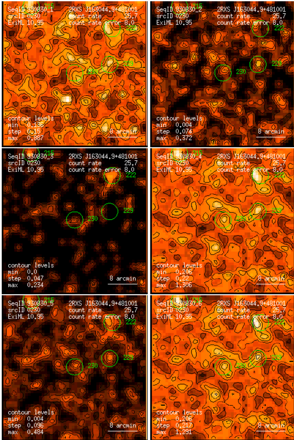
Figure 230: RASS 930830: detection 0230: band rate images, Gaussian filter: (1) PSPC channels 11 – 41, (2) 52 – 90, (3) 91 – 201, (4) 11 – 235, (5) 52 – 201, (6) 11 – 201. Broad band rates in counts/ks. Band rate contour levels in counts/ks/arcmin 2 .
