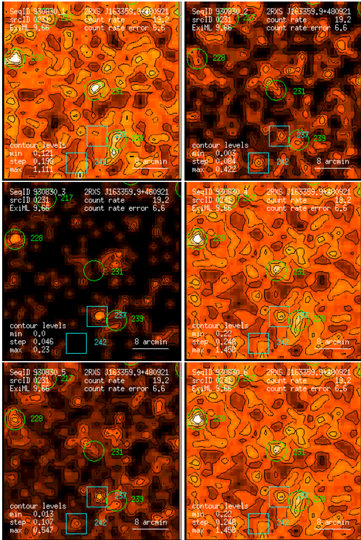
Figure 231: RASS 930830: detection 0231: band rate images, Gaussian filter: (1) PSPC channels 11 – 41, (2) 52 – 90, (3) 91 – 201, (4) 11 – 235, (5) 52 – 201, (6) 11 – 201. Broad band rates in counts/ks. Band rate contour levels in counts/ks/arcmin 2 .
