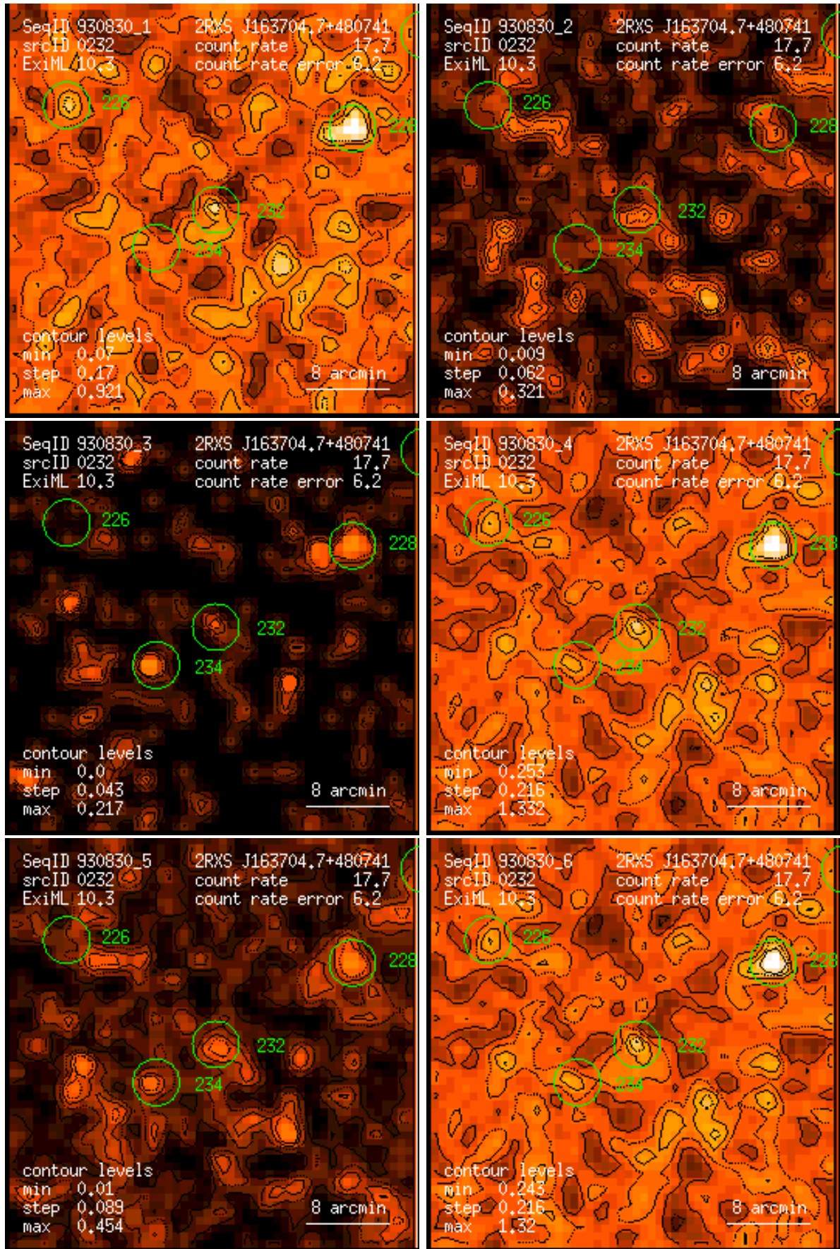
Figure 232: RASS 930830: detection 0232: band rate images, Gaussian filter: (1) PSPC channels 11 – 41, (2) 52 – 90, (3) 91 – 201, (4) 11 – 235, (5) 52 – 201, (6) 11 – 201. Broad band rates in counts/ks. Band rate contour levels in counts/ks/arcmin 2 .
