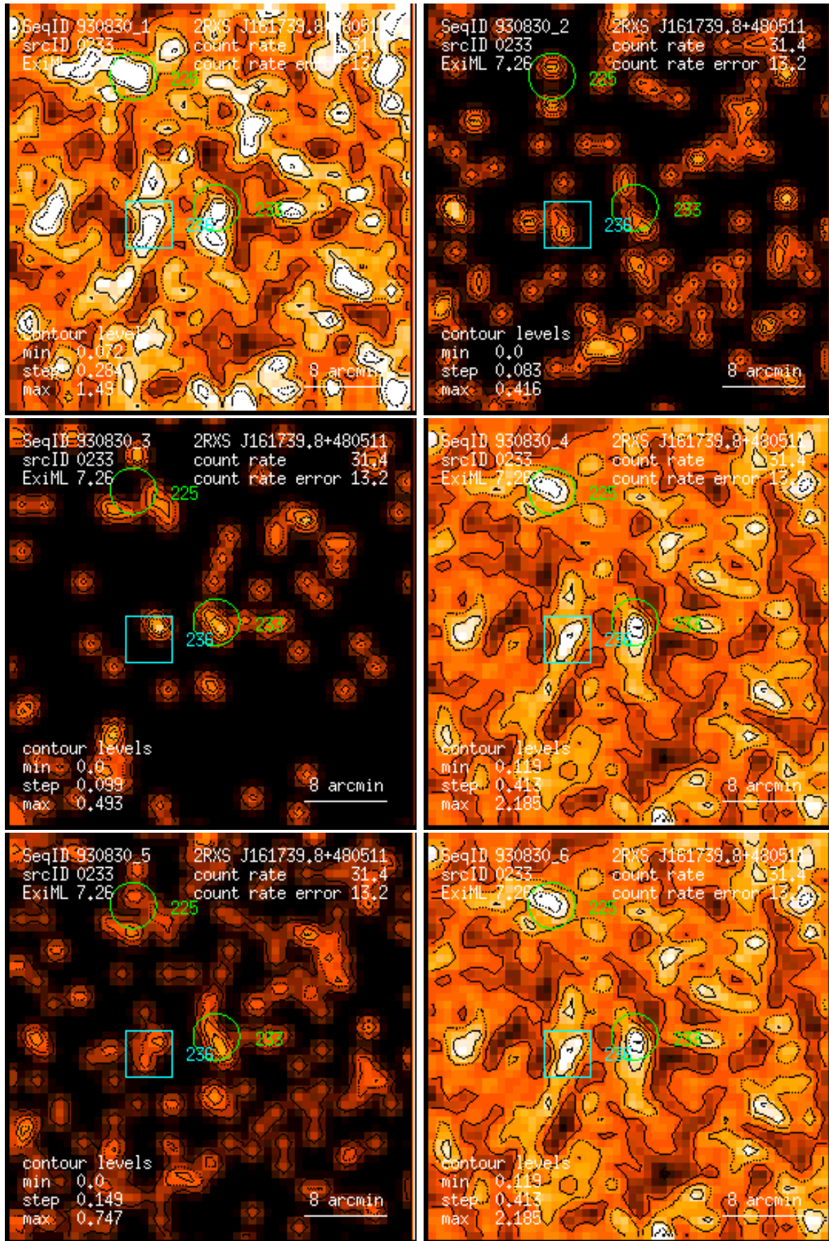
Figure 233: RASS 930830: detection 0233: band rate images, Gaussian filter: (1) PSPC channels 11 – 41, (2) 52 – 90, (3) 91 – 201, (4) 11 – 235, (5) 52 – 201, (6) 11 – 201. Broad band rates in counts/ks. Band rate contour levels in counts/ks/arcmin 2 .
