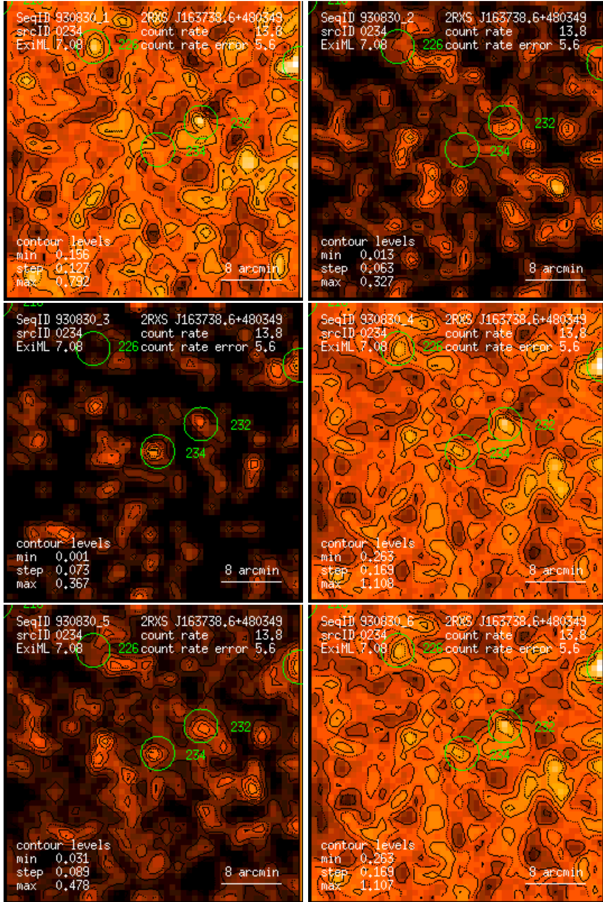
Figure 234: RASS 930830: detection 0234: band rate images, Gaussian filter: (1) PSPC channels 11 – 41, (2) 52 – 90, (3) 91 – 201, (4) 11 – 235, (5) 52 – 201, (6) 11 – 201. Broad band rates in counts/ks. Band rate contour levels in counts/ks/arcmin 2 .
