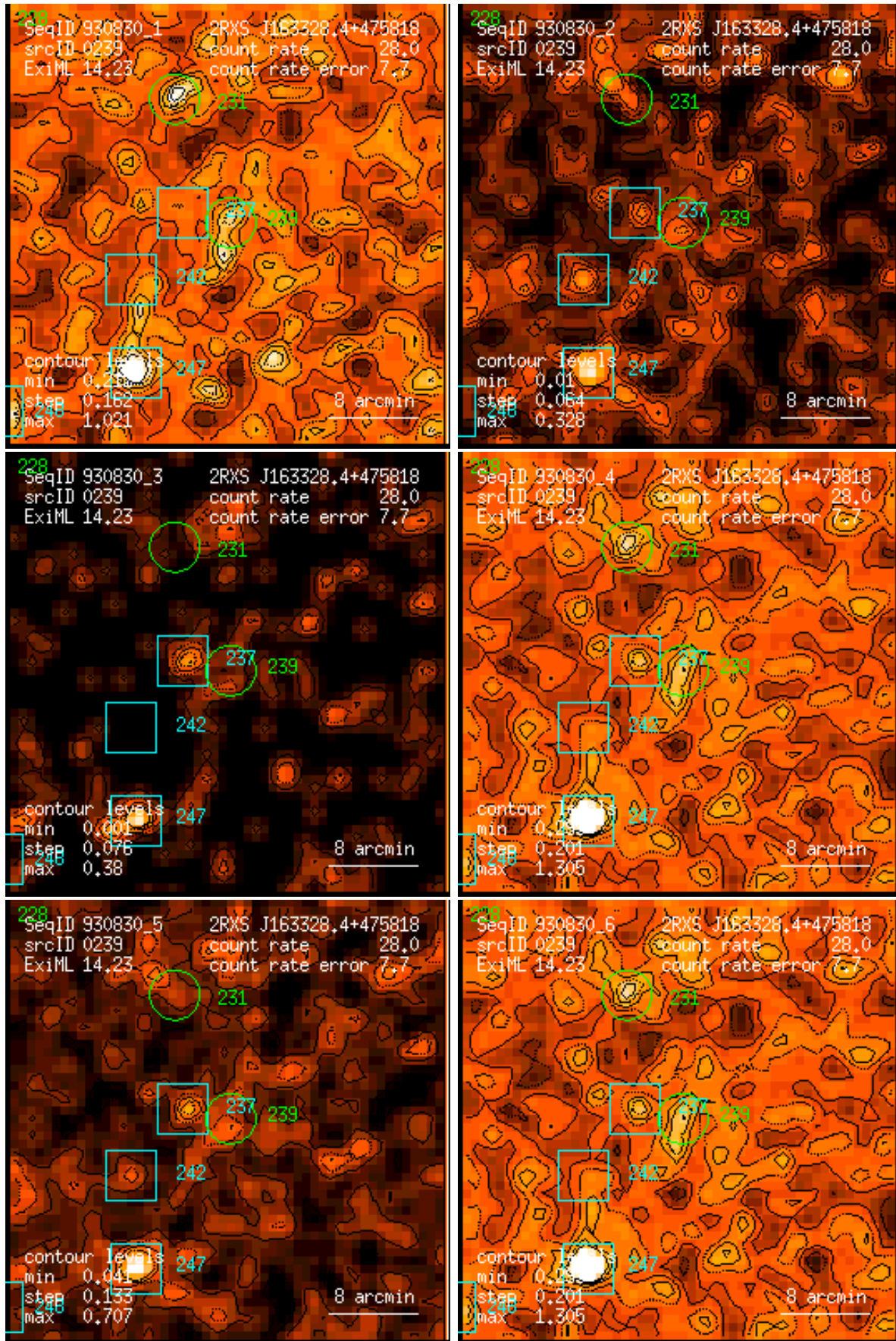
Figure 239: RASS 930830: detection 0239: band rate images, Gaussian filter: (1) PSPC channels 11 – 41, (2) 52 – 90, (3) 91 – 201, (4) 11 – 235, (5) 52 – 201, (6) 11 – 201. Broad band rates in counts/ks. Band rate contour levels in counts/ks/arcmin 2 .
