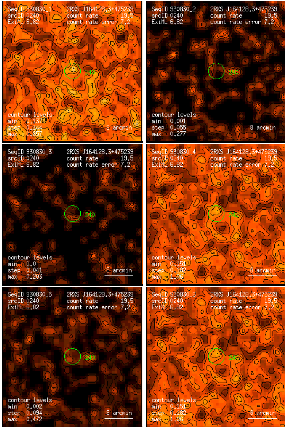
Figure 240: RASS 930830: detection 0240: band rate images, Gaussian filter: (1) PSPC channels 11 – 41, (2) 52 – 90, (3) 91 – 201, (4) 11 – 235, (5) 52 – 201, (6) 11 – 201. Broad band rates in counts/ks. Band rate contour levels in counts/ks/arcmin 2 .
