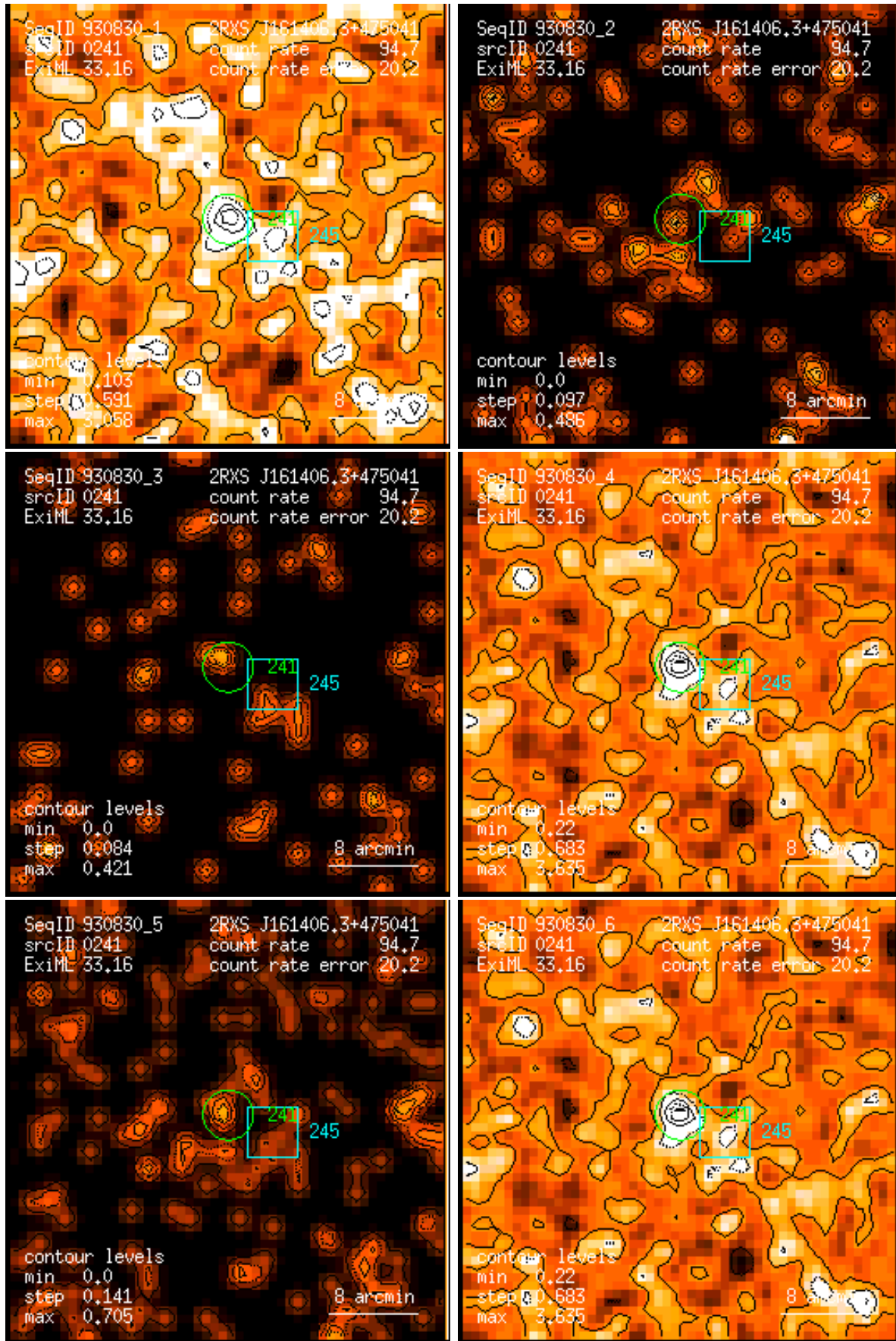
Figure 241: RASS 930830: detection 0241: band rate images, Gaussian filter: (1) PSPC channels 11 – 41, (2) 52 – 90, (3) 91 – 201, (4) 11 – 235, (5) 52 – 201, (6) 11 – 201. Broad band rates in counts/ks. Band rate contour levels in counts/ks/arcmin 2 .
