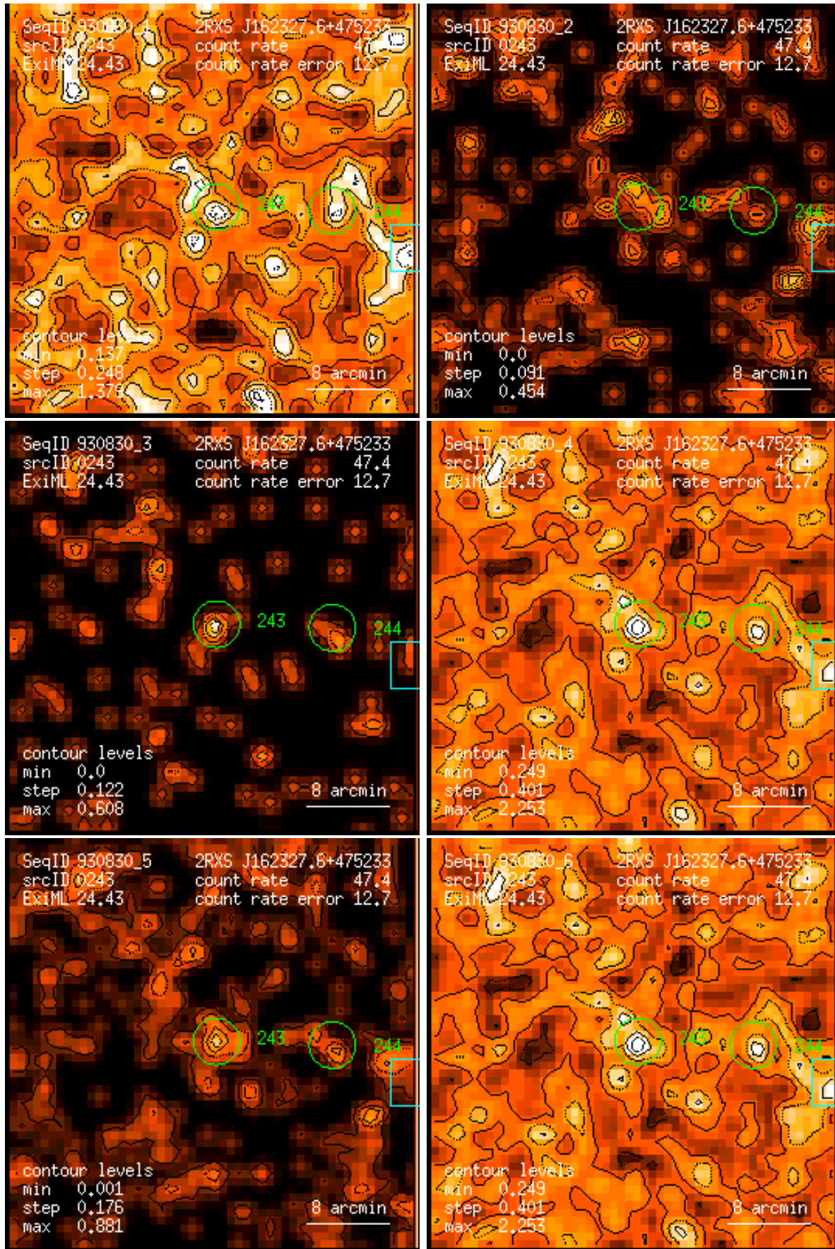
Figure 243: RASS 930830: detection 0243: band rate images, Gaussian filter: (1) PSPC channels 11 – 41, (2) 52 – 90, (3) 91 – 201, (4) 11 – 235, (5) 52 – 201, (6) 11 – 201. Broad band rates in counts/ks. Band rate contour levels in counts/ks/arcmin 2 .
