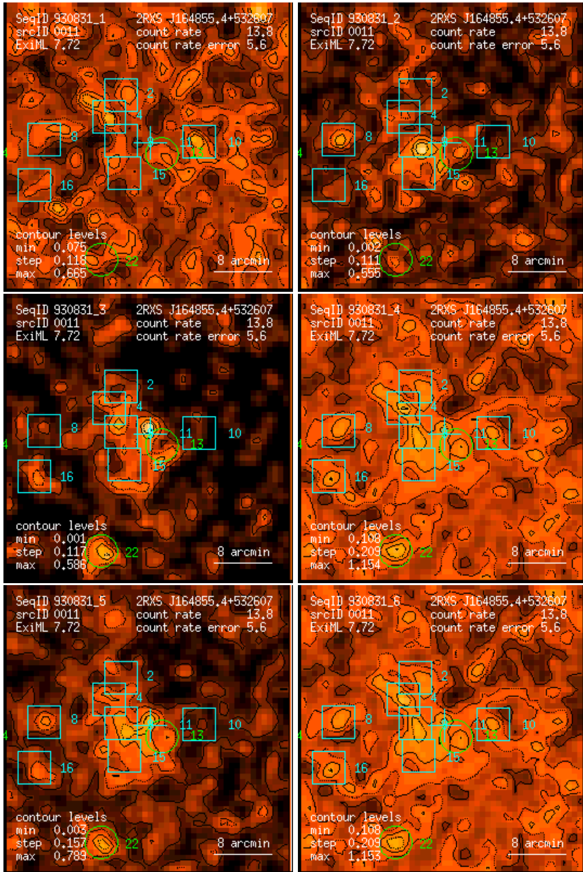
Figure 11: RASS 930831: detection 0011: band rate images, Gaussian filter: (1) PSPC channels 11 – 41, (2) 52 – 90, (3) 91 – 201, (4) 11 – 235, (5) 52 – 201, (6) 11 – 201. Broad band rates in counts/ks. Band rate contour levels in counts/ks/arcmin 2 .
