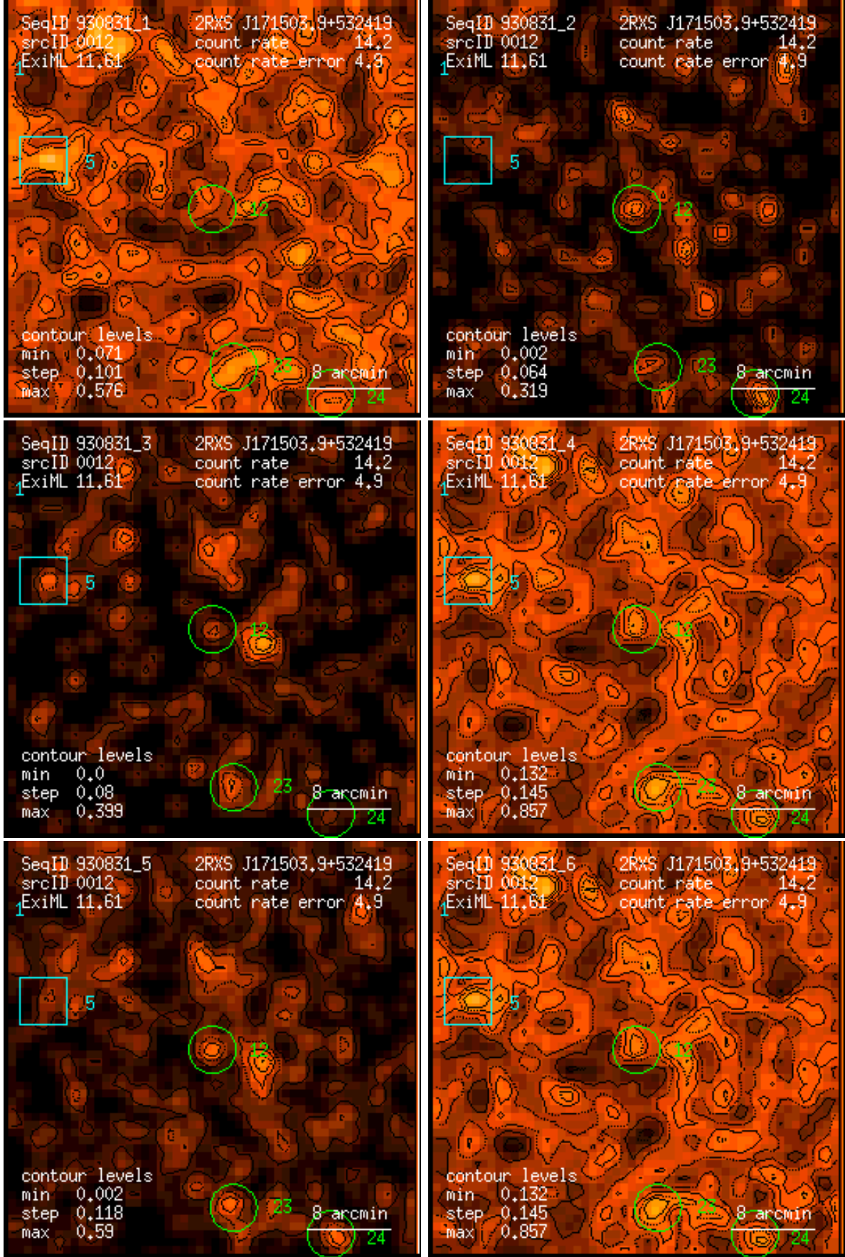
Figure 12: RASS 930831: detection 0012: band rate images, Gaussian filter: (1) PSPC channels 11 – 41, (2) 52 – 90, (3) 91 – 201, (4) 11 – 235, (5) 52 – 201, (6) 11 – 201. Broad band rates in counts/ks. Band rate contour levels in counts/ks/arcmin 2 .
