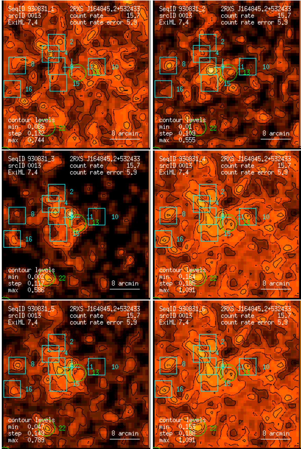
Figure 13: RASS 930831: detection 0013: band rate images, Gaussian filter: (1) PSPC channels 11 – 41, (2) 52 – 90, (3) 91 – 201, (4) 11 – 235, (5) 52 – 201, (6) 11 – 201. Broad band rates in counts/ks. Band rate contour levels in counts/ks/arcmin 2 .
