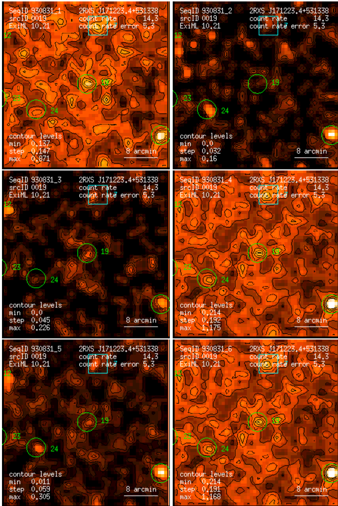
Figure 19: RASS 930831: detection 0019: band rate images, Gaussian filter: (1) PSPC channels 11 – 41, (2) 52 – 90, (3) 91 – 201, (4) 11 – 235, (5) 52 – 201, (6) 11 – 201. Broad band rates in counts/ks. Band rate contour levels in counts/ks/arcmin 2 .
