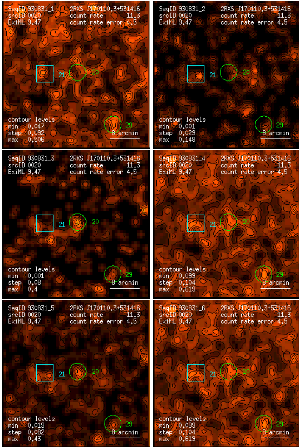
Figure 20: RASS 930831: detection 0020: band rate images, Gaussian filter: (1) PSPC channels 11 – 41, (2) 52 – 90, (3) 91 – 201, (4) 11 – 235, (5) 52 – 201, (6) 11 – 201. Broad band rates in counts/ks. Band rate contour levels in counts/ks/arcmin 2 .
